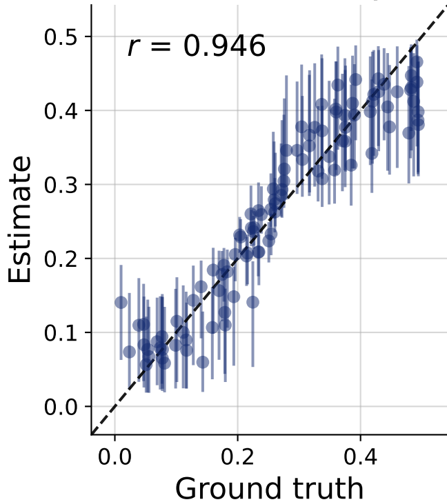
Network Density \delta
