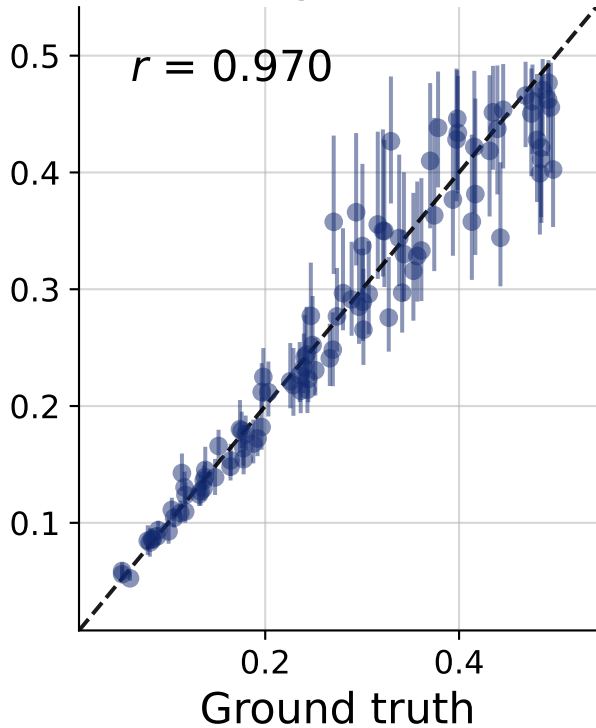
Exchange Factor \alpha
