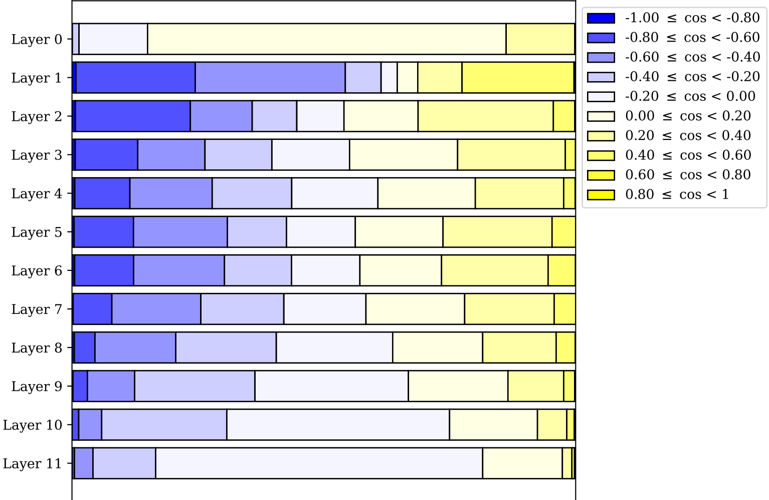
gpt2-small
