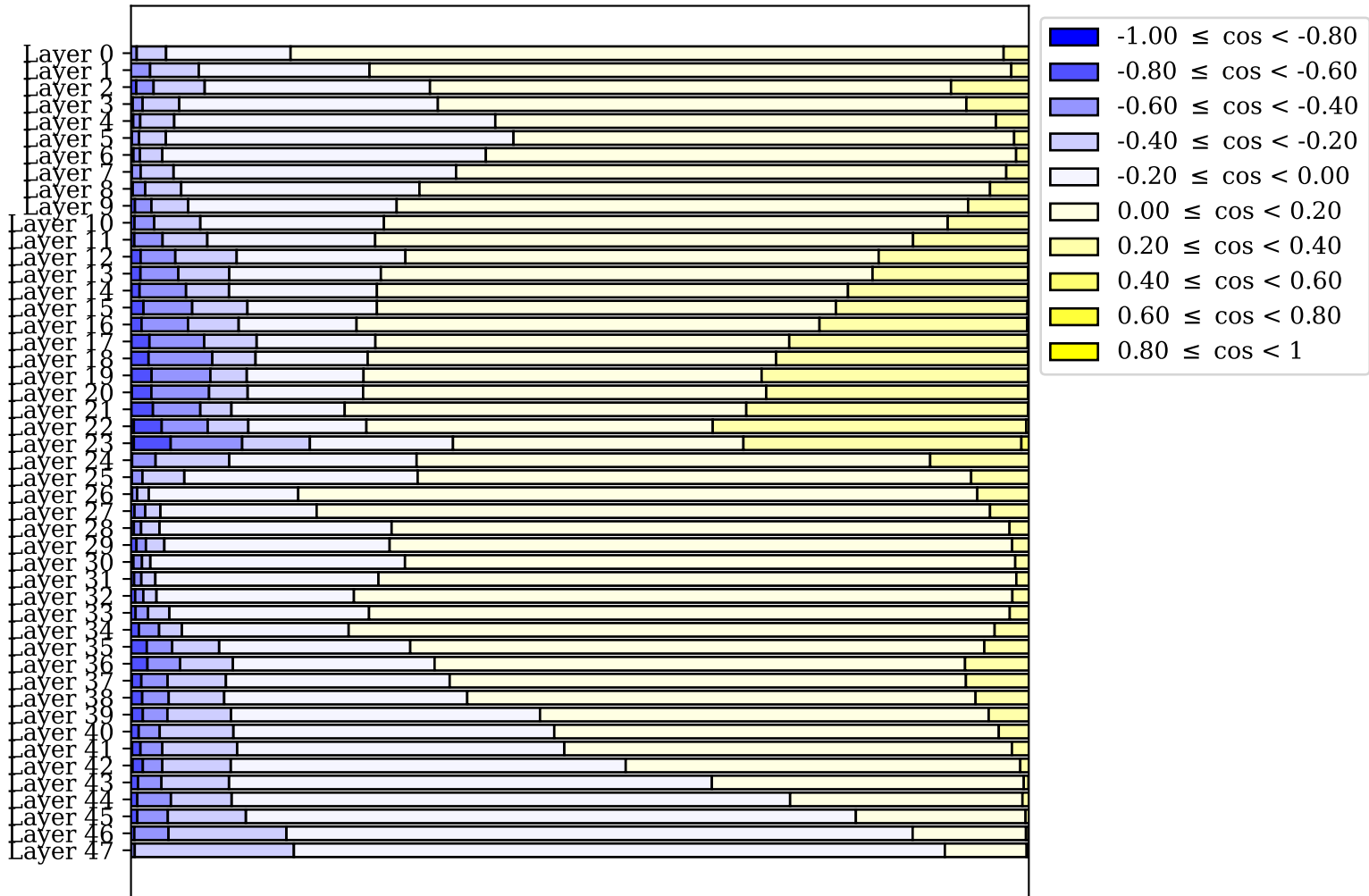
t5-large
