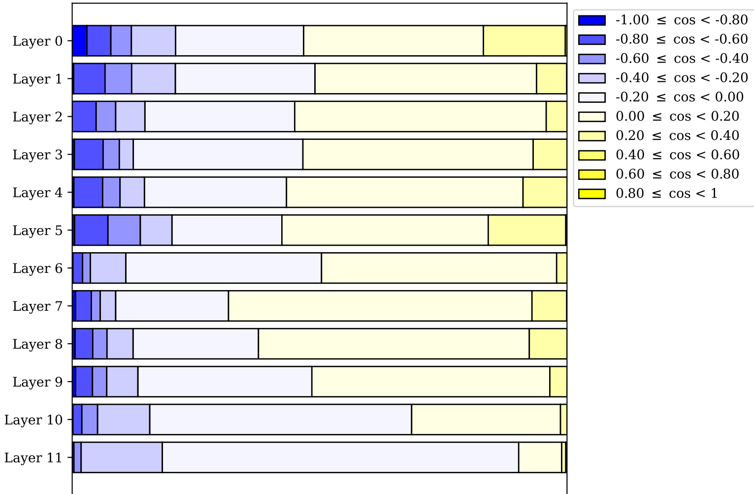
t5-small
