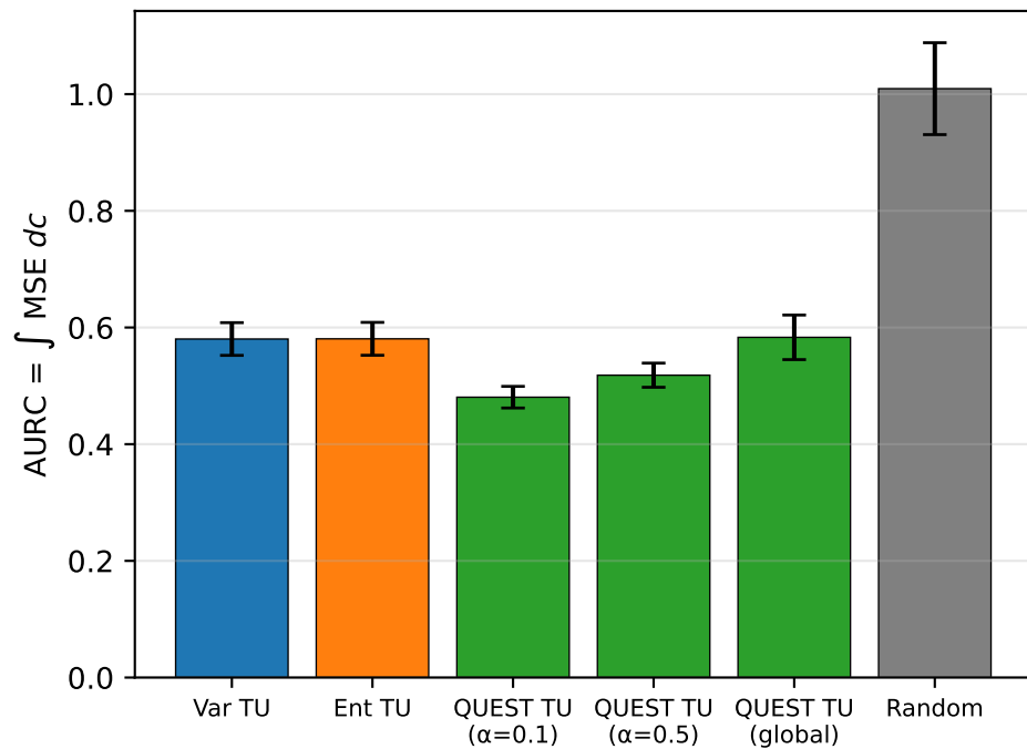
t5 ( n_{seeds}=10 )
