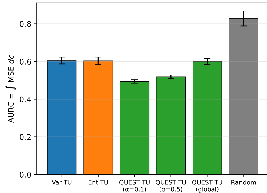
gaussian ( n_{seeds}=10 )
