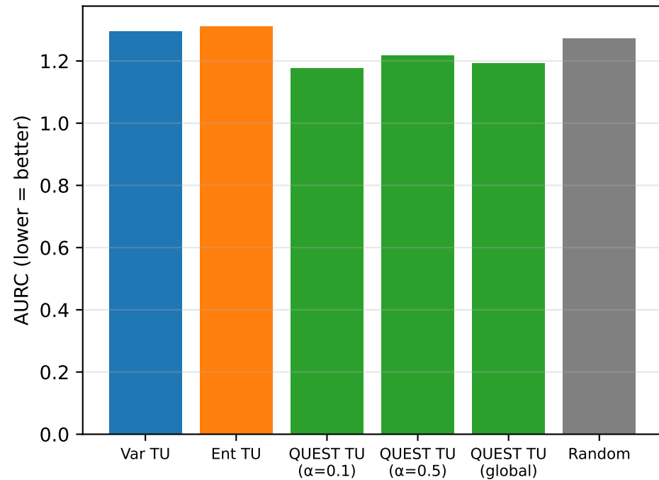
Noise: gaussian
