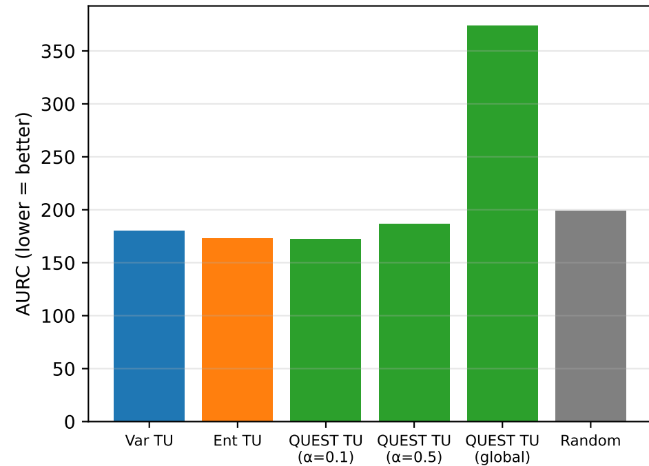
Noise: t1
