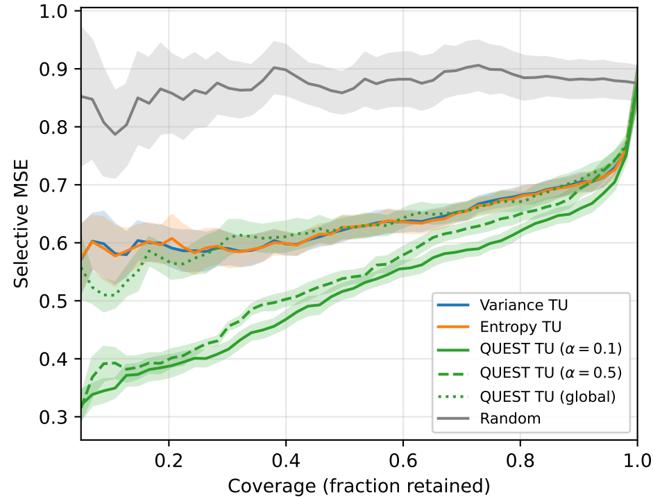
gaussian (full MSE = 0.875 \pm 0.030 , n_{seeds}=10 )
