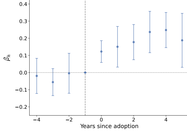
Figure 1: Excess probabilities.
