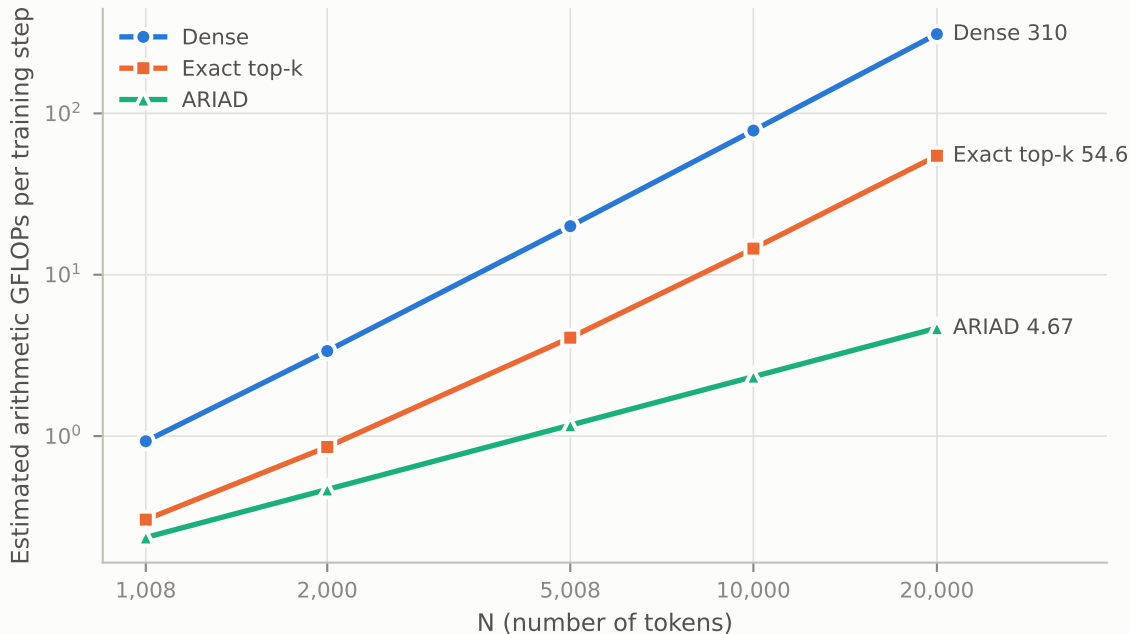
Estimated training FLOPs vs N (dual-space QK, k=32, sparse top-32 teacher)
