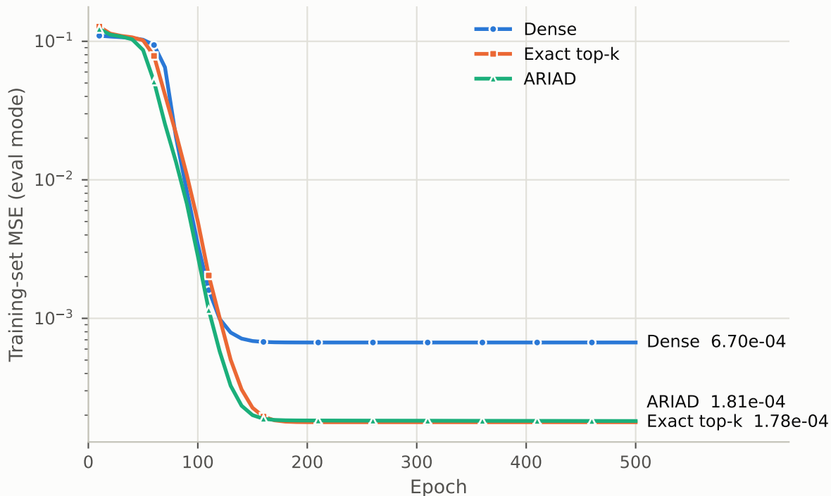
MSE convergence (N=10,000, k=32, sparse top-32 teacher)
