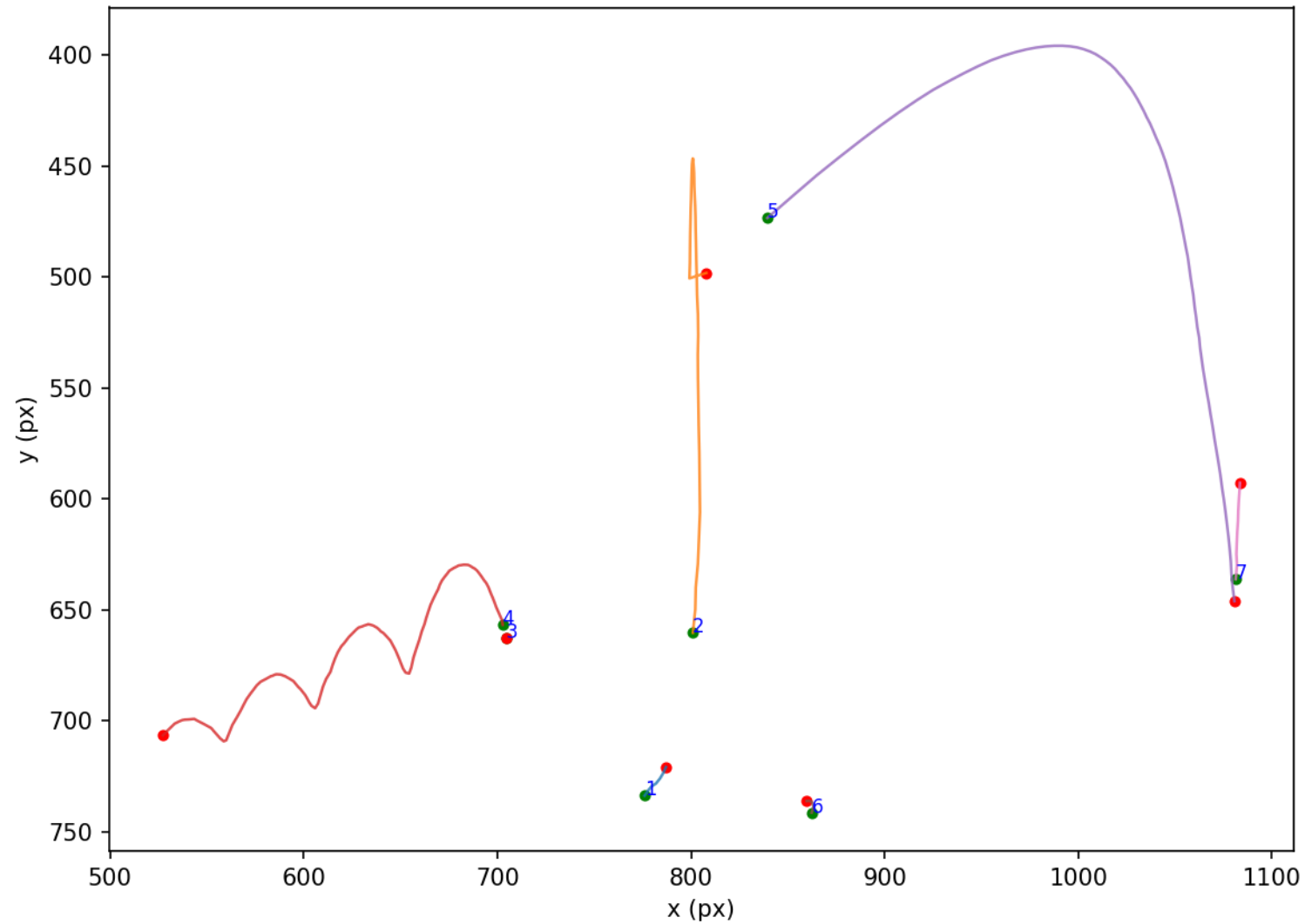
Before Merge: Raw SORT Tracks
