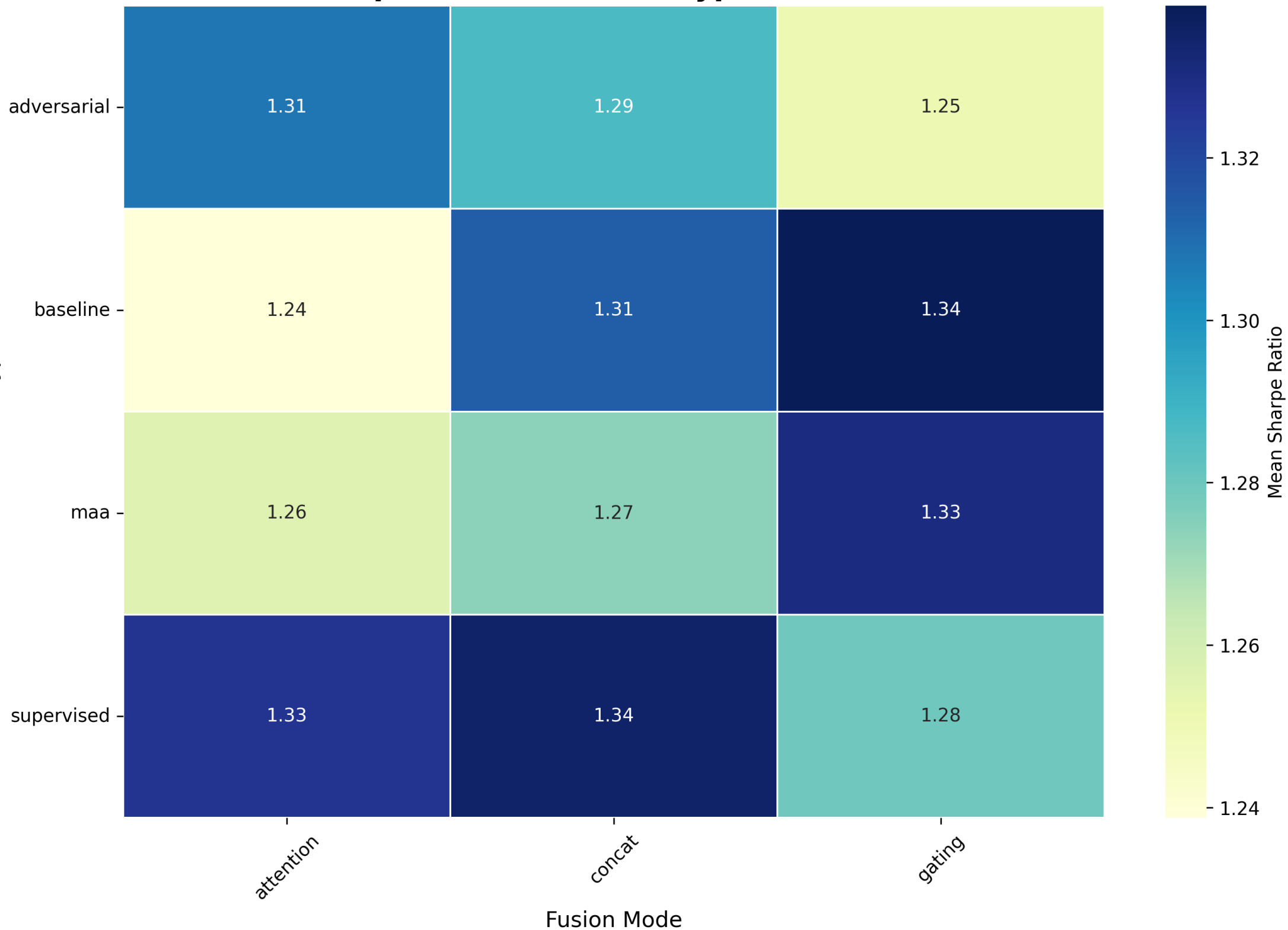
Mean Sharpe Ratio: Pretrain Type vs. Fusion Mode
