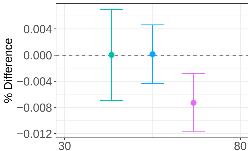
Mean and standard error of estimated vs. true prevalence
