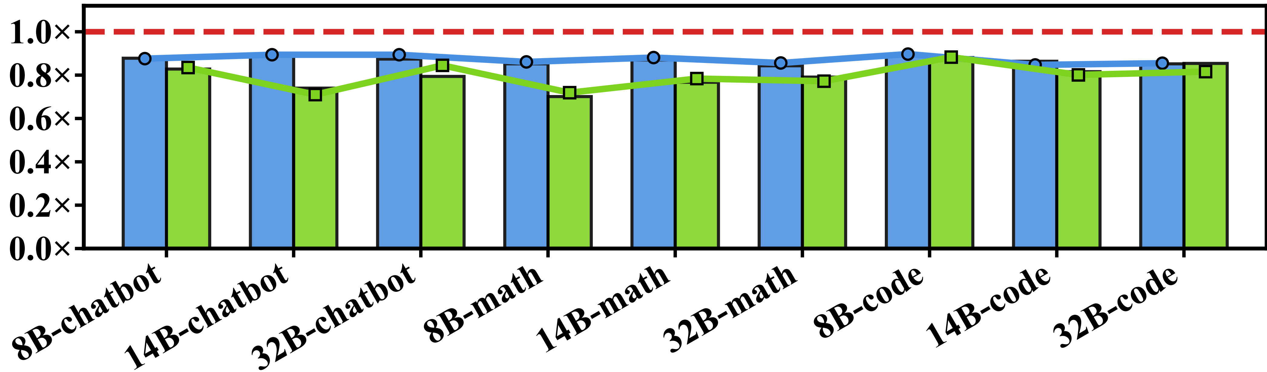
Normalized Performance
