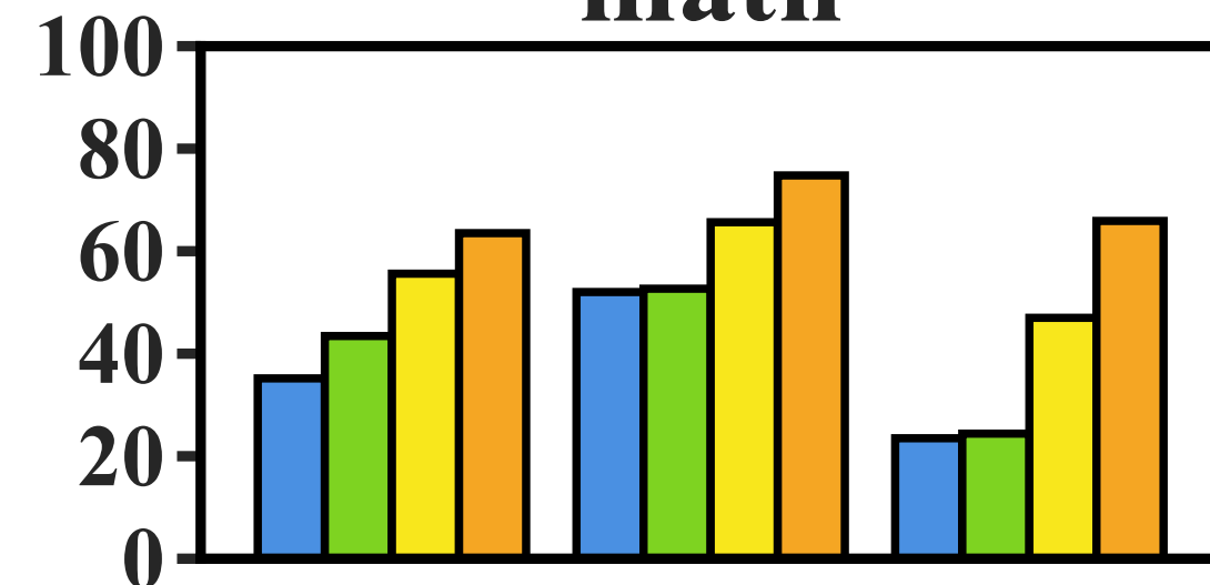
math
