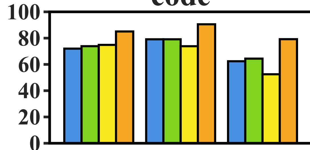
code
