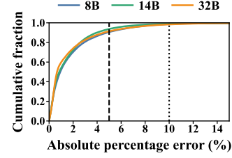
Fig. 11. CDF of the step-time model's absolute percentage error for the three models.
