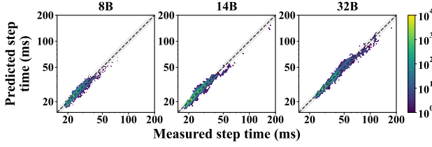
Fig. 10. Predicted versus measured step time for the three models. The dashed line denotes equal predicted and measured times. Color represents the number of steps per hexagon on a logarithmic scale.
