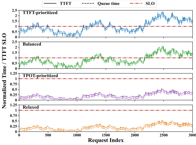
Fig. 2. Normalized TTFT and queueing time under FCFS.
