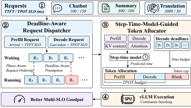
Fig. 4. Design overview of TANGO.
