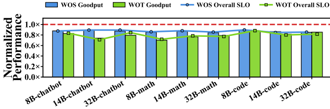
Fig. 9. The goodput and overall SLO attainment of TANGO’s variants normalized to TANGO, represented by bars and curves, respectively.
