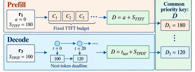
Fig. 5. Phase-aware deadlines for request prioritization (times in ms).
