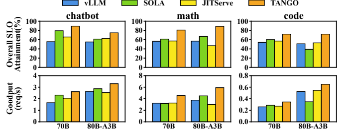
Fig. 13. The overall SLO attainment and goodput of TANGO, vLLM, SOLA, and JITServe with the 70B and 80B-A3B models on the three workloads.
