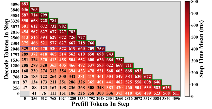
Fig. 3. Mean step time with different prefill and decode token counts.
