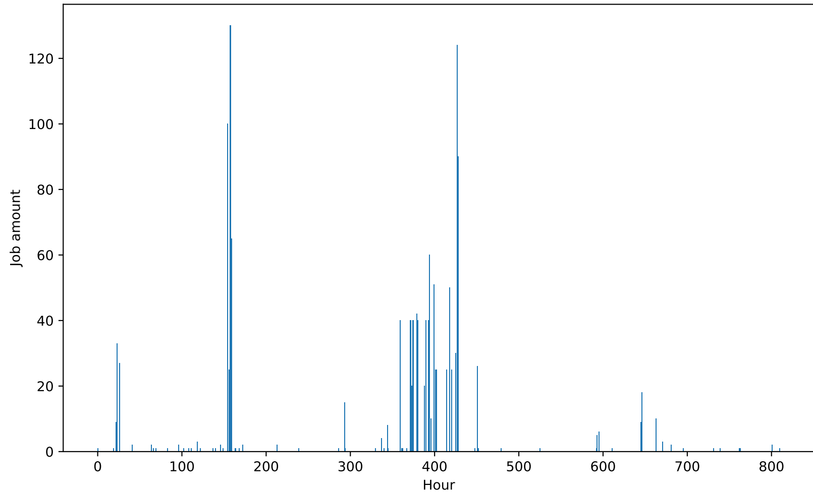
Distribution of Job Submission Time
