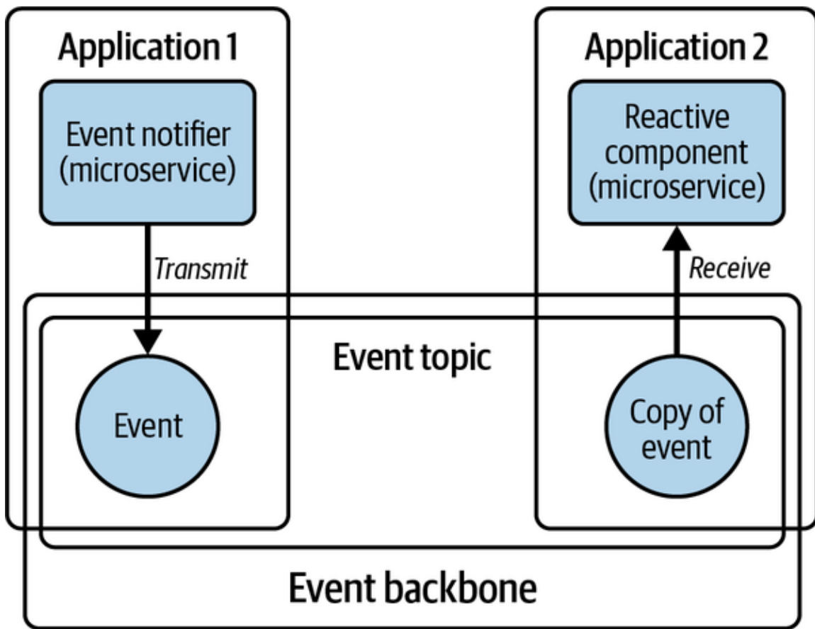
Figure 6-4. Event Choreography pattern
