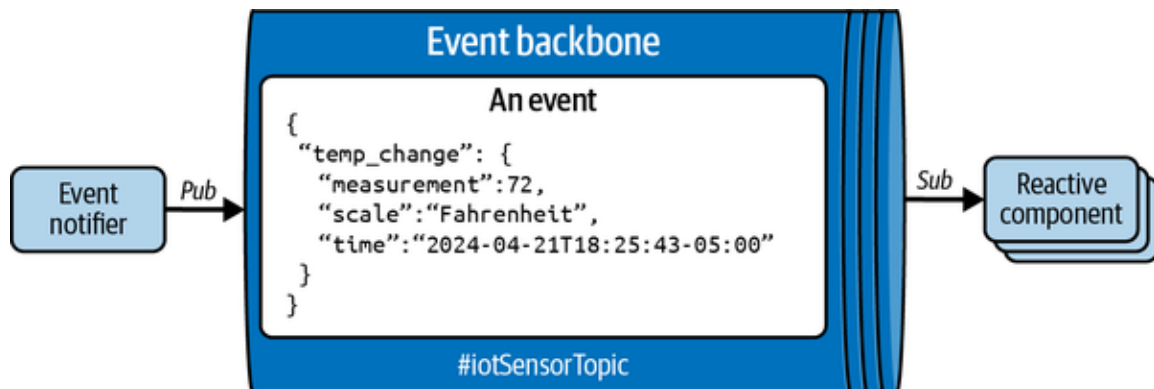
Figure 6-7. Event in transit
