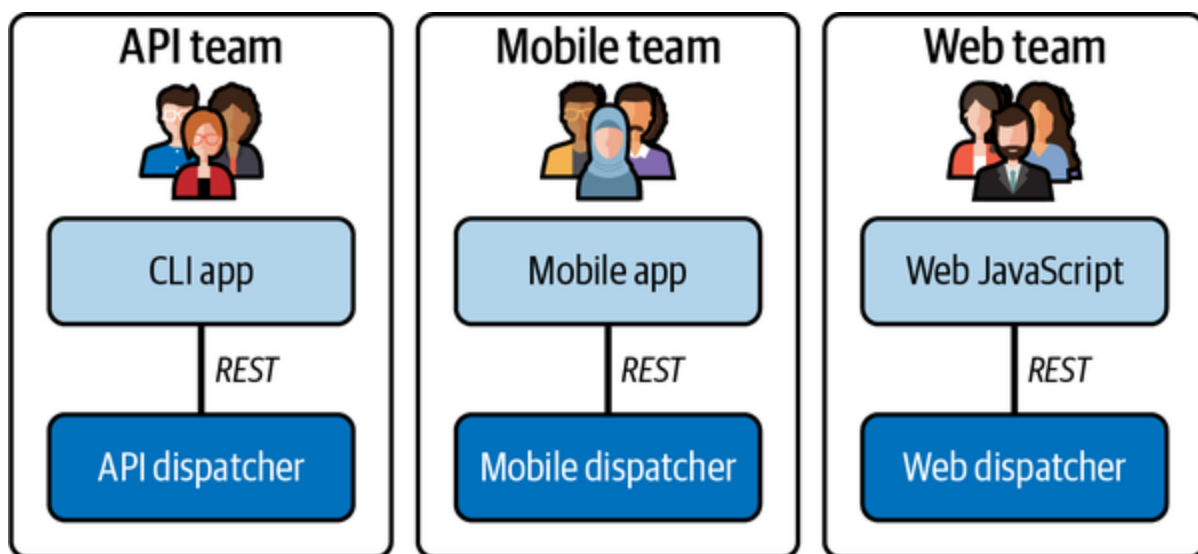
Figure 4-16. Dispatcher teams
