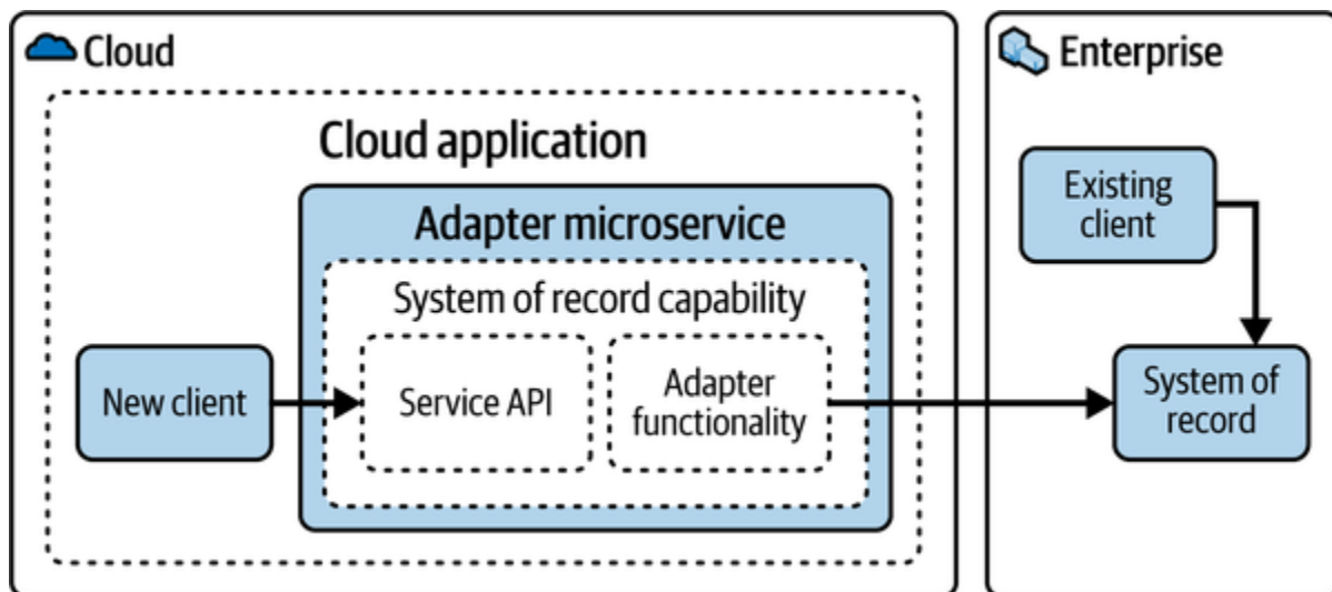
Figure 4-12. Adapter Microservice
