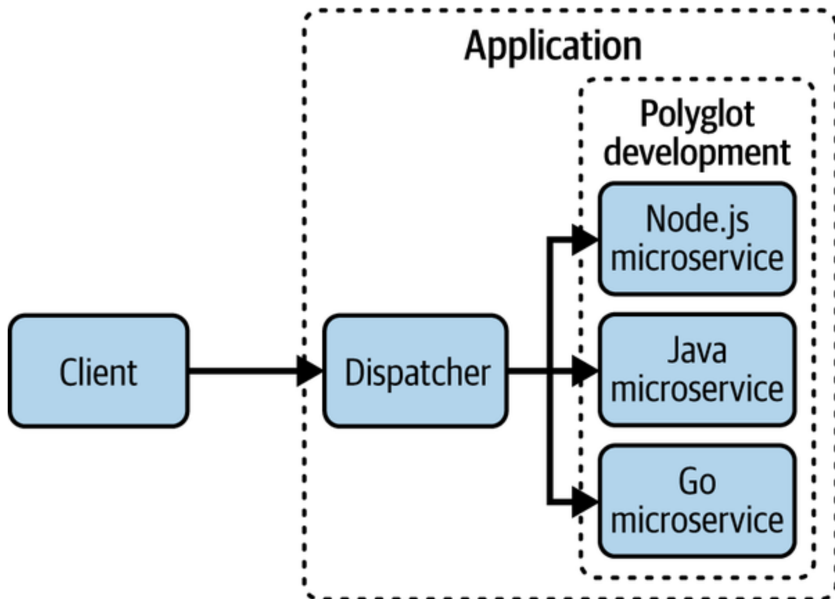
Figure 4-18. Polyglot Development
