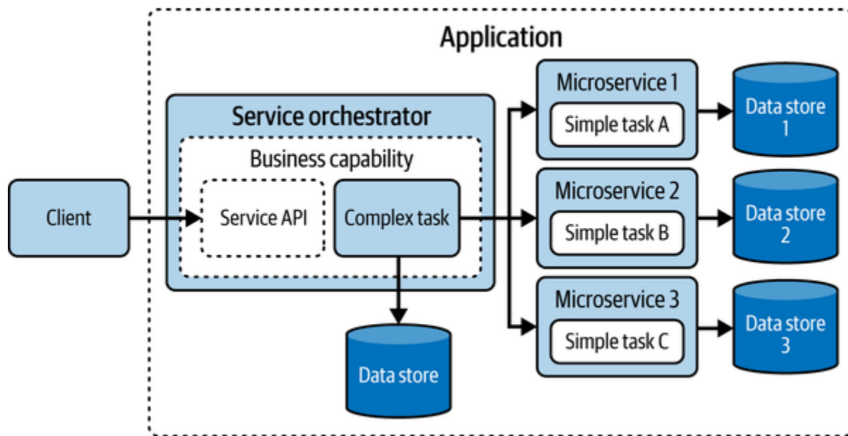
Figure 4-24. Service Orchestrator
