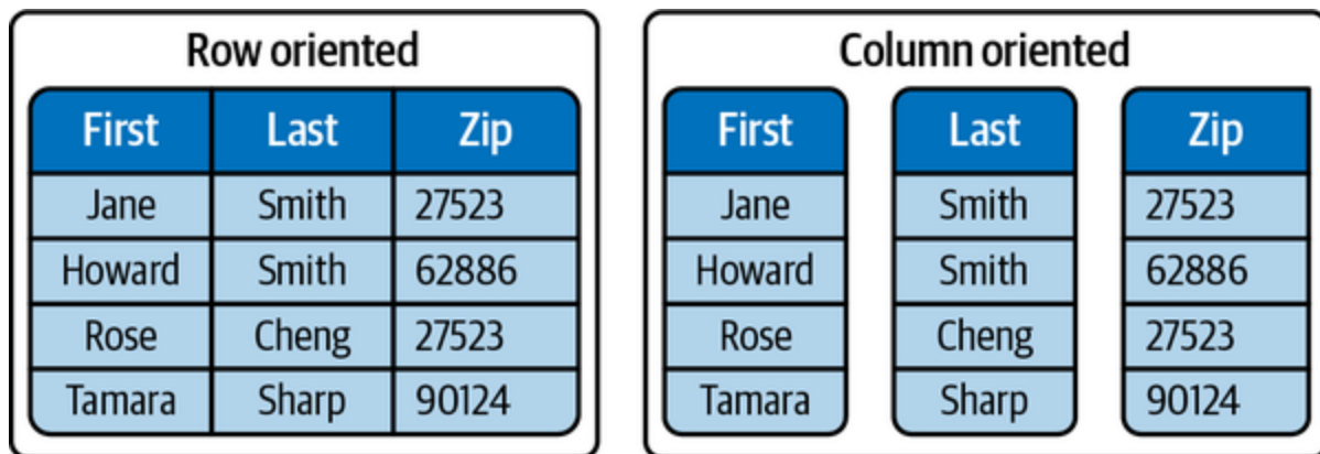
Figure 7-21. Column orientation
