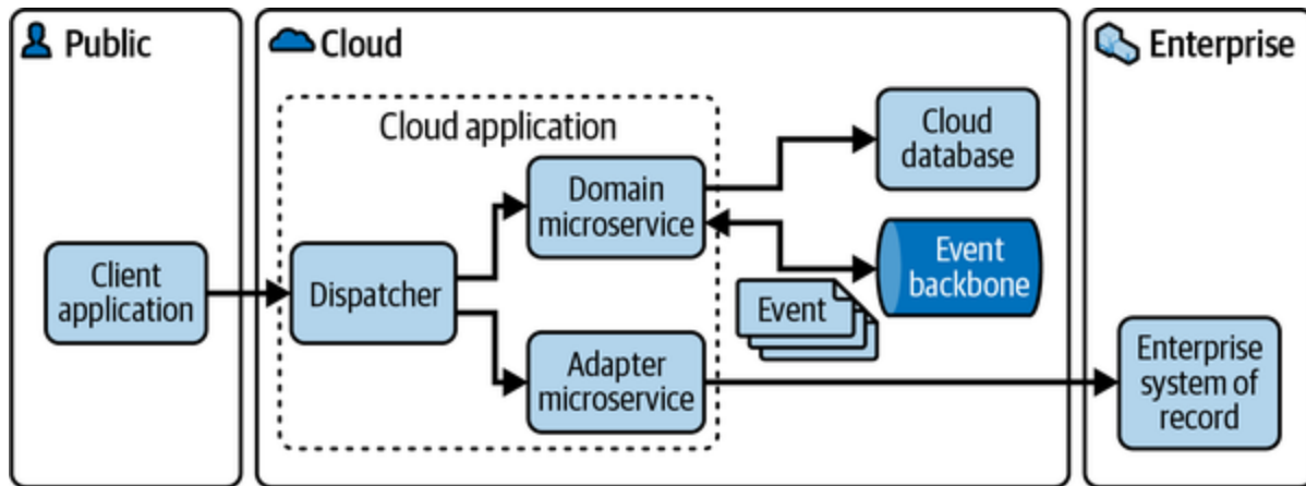
Figure 1-1. Cloud Application
