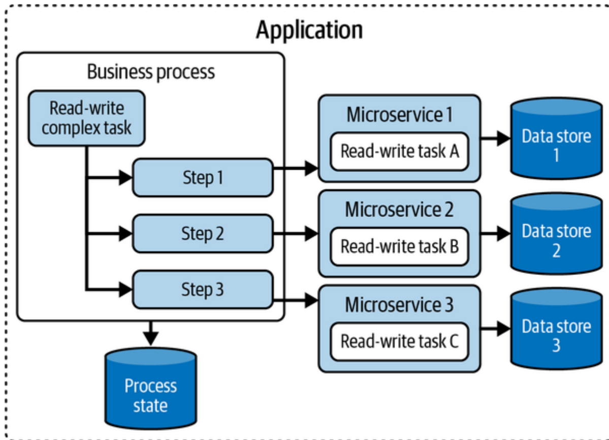
Figure 4-27. Business process
