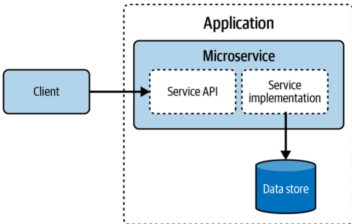
Figure 4-4. Microservice
