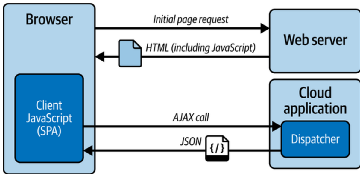
Figure 8-14. AJAX interactions
