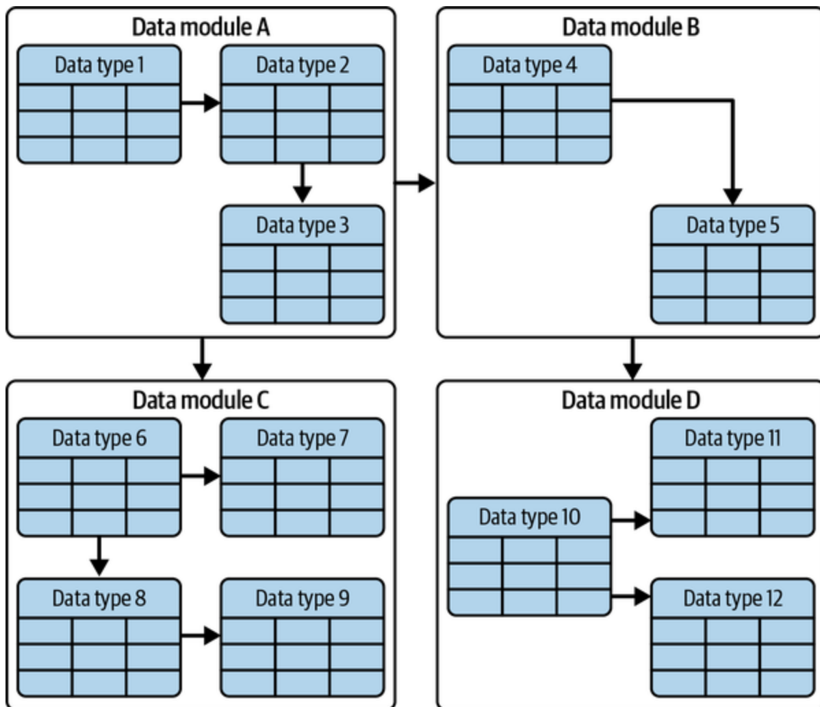
Figure 7-25. Data Module
