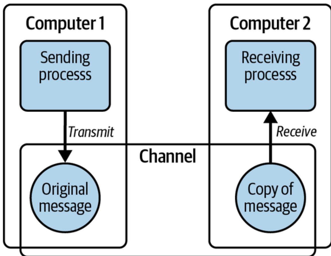
Figure 6-3. Messaging pattern
