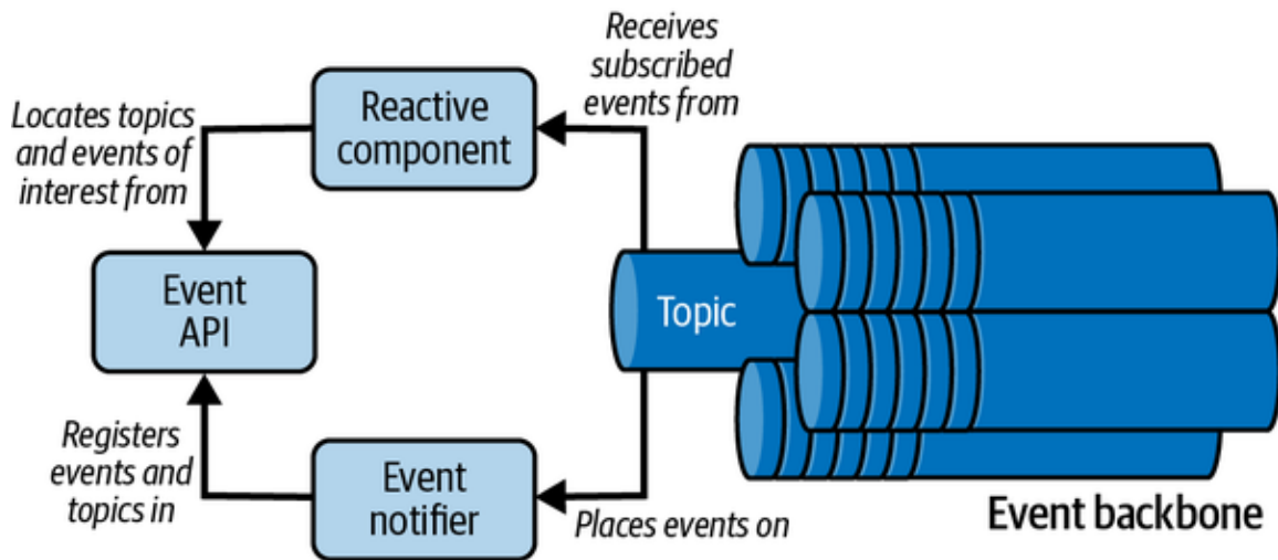
Figure 6-19. Event Backbone
