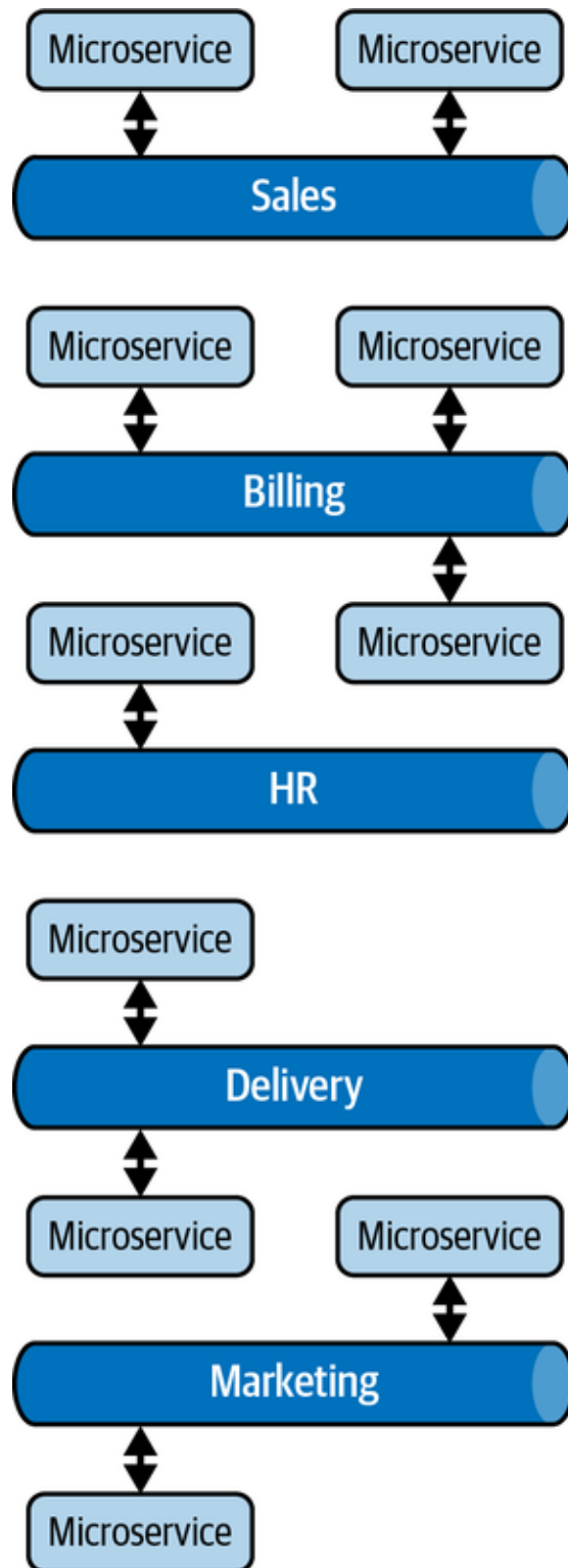
Figure 6-22. Multiple backbones
