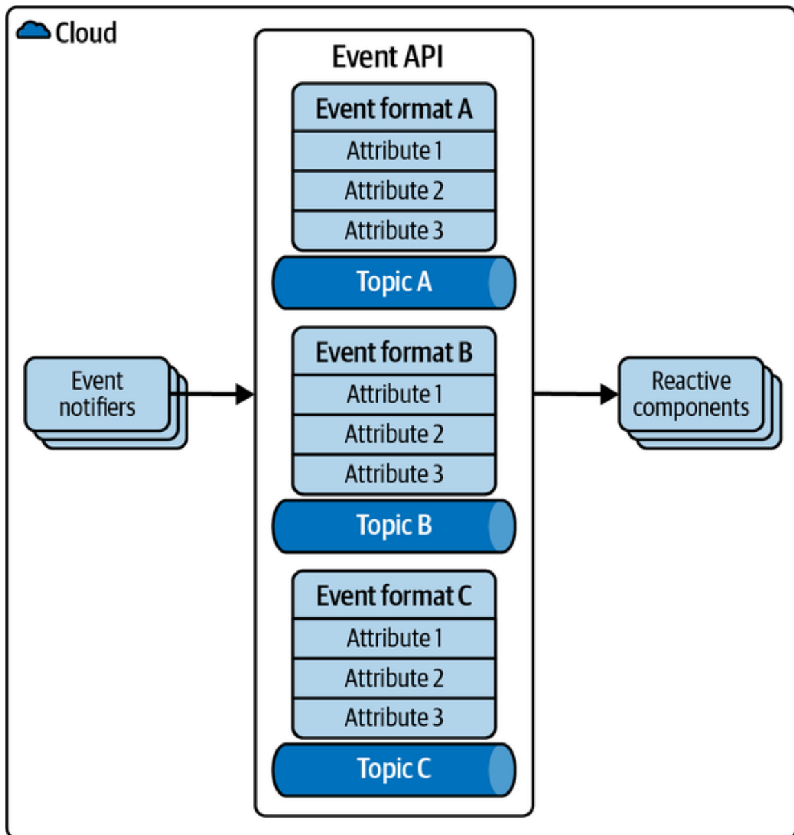
Figure 6-16. Event API
