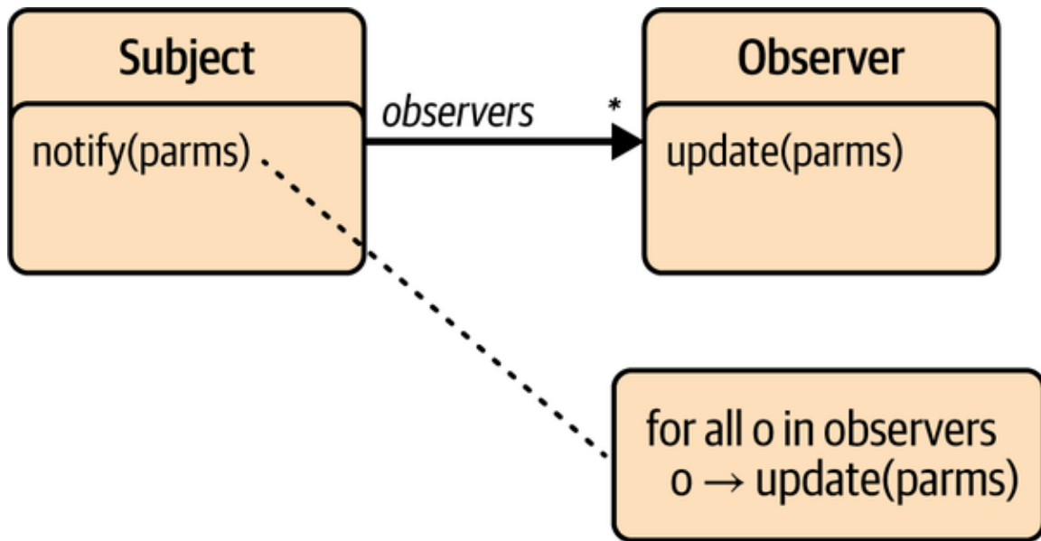
Figure 6-2. Observer pattern
