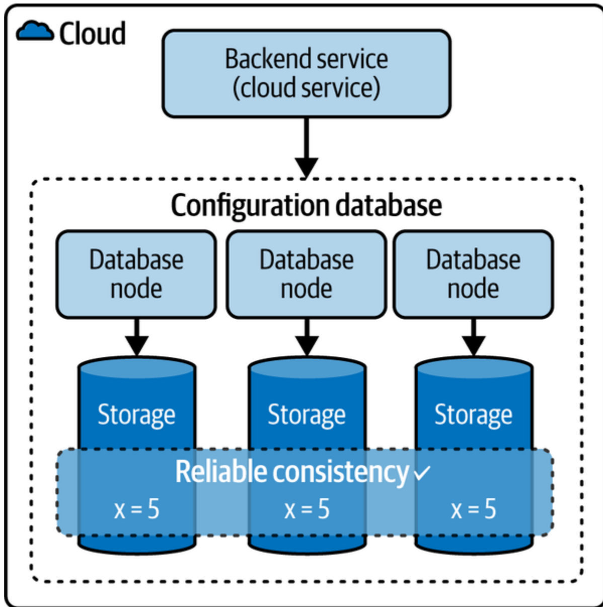
Figure 7-12. Configuration Database
