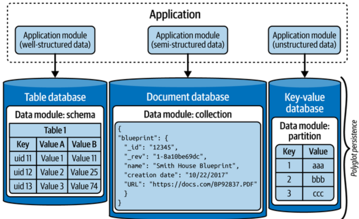
Figure 7-30. Polyglot Persistence
