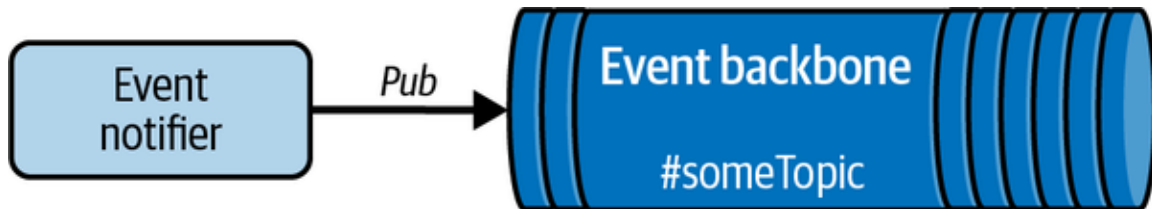
Figure 6-14. Event Notifier
