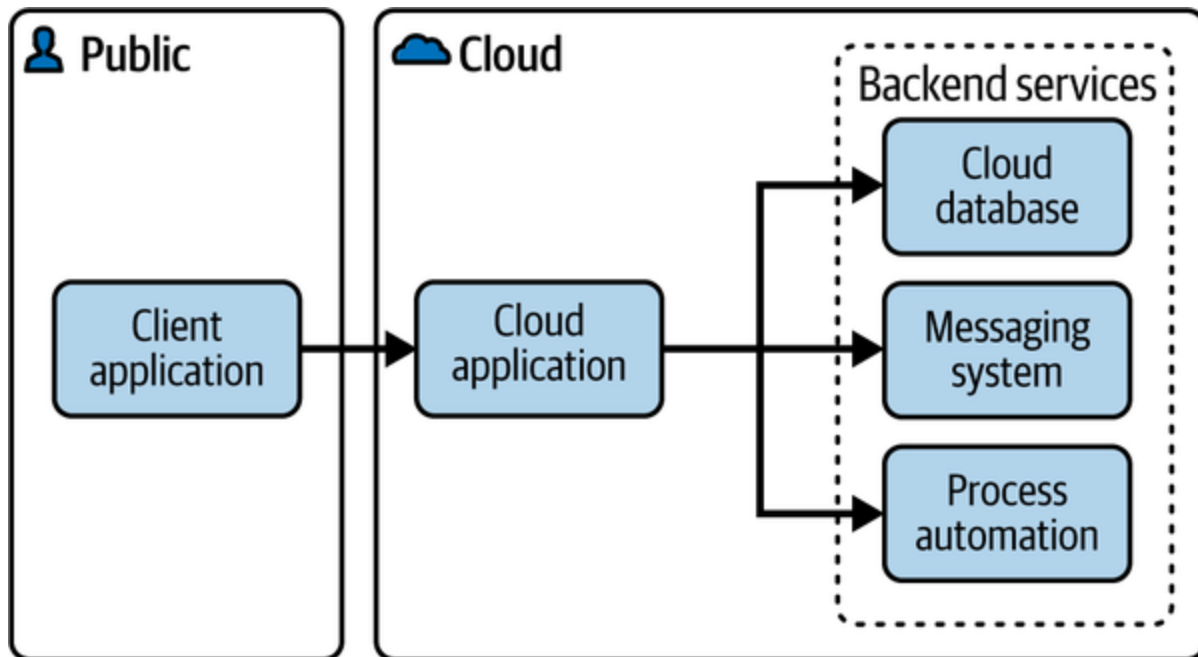
Figure 3-15. Backend Services
