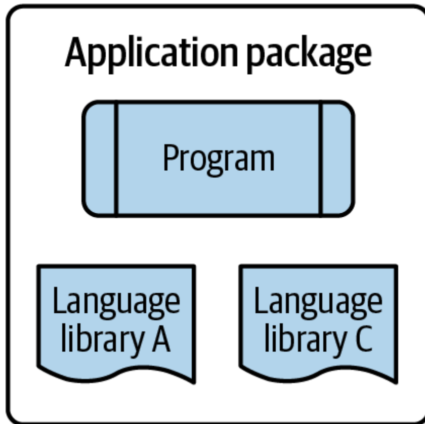
Figure 3-4. Application Package
