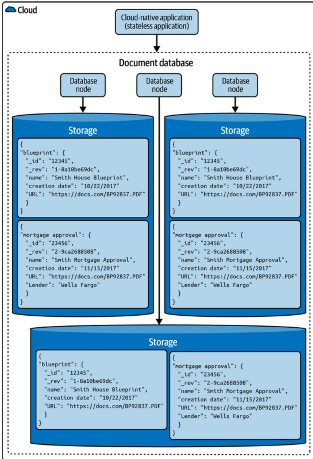
Figure 7-15. Document Database
