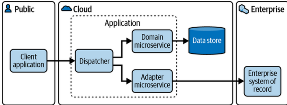
Figure 4-5. Microservices application
