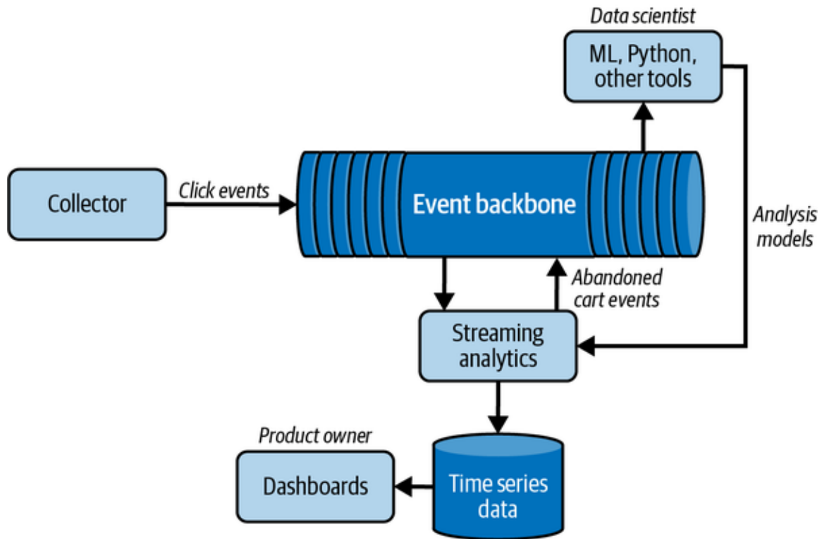
Figure 6-8. Clickstream analytics
