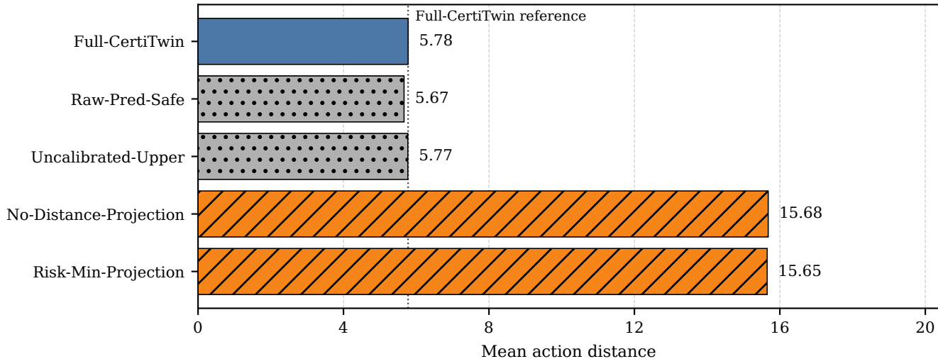
Action-distance comparison under ablation variants
