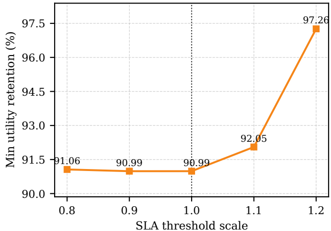
(b) Utility retention under SLA shifts
