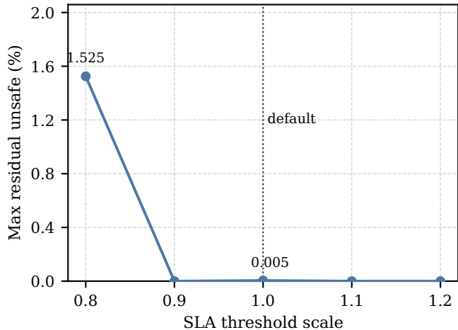
(a) Residual unsafe rate under SLA shifts
