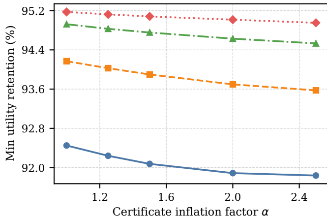
(b) Utility-retention tradeoff
