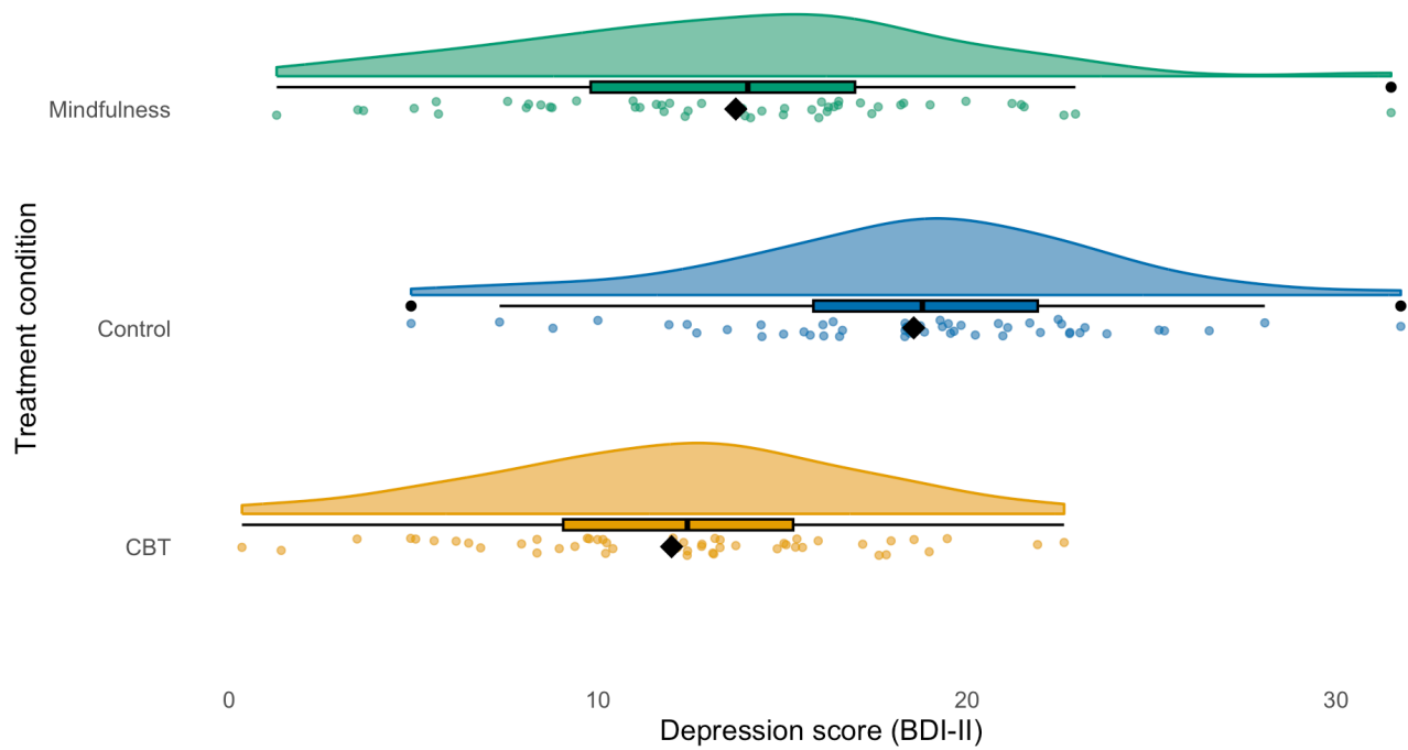
Post-Treatment Depression by Condition Diamond = mean. Density = distribution. Box = IQR. Dots = individual scores.
