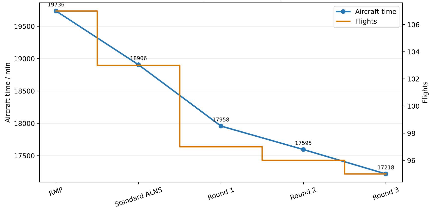
Q2: exact local repair, restarts and absorption
