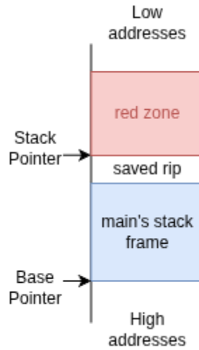
Figure 1.10: Example of function call that does not allocate space of the stack but access the variable saved on the red zone
