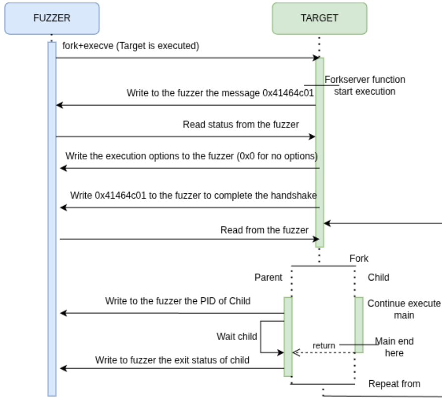
Figure 1.12: AFL++ Forkserver Protocol
