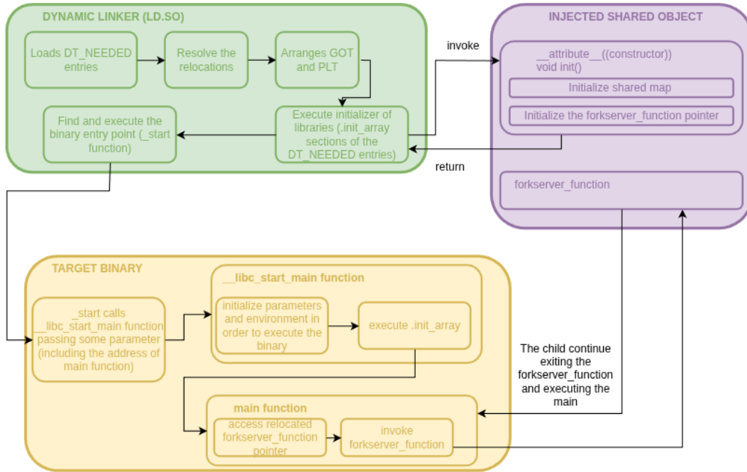
Figure 2.4: Optimized forklserver invocation
