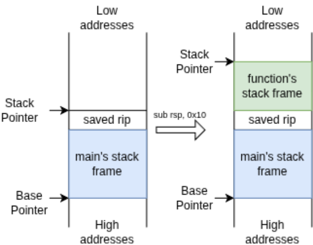
Figure 1.9: Example of what happend during a function call in case of frame pointer omission
