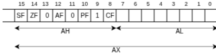
(b) ax register after lahf
