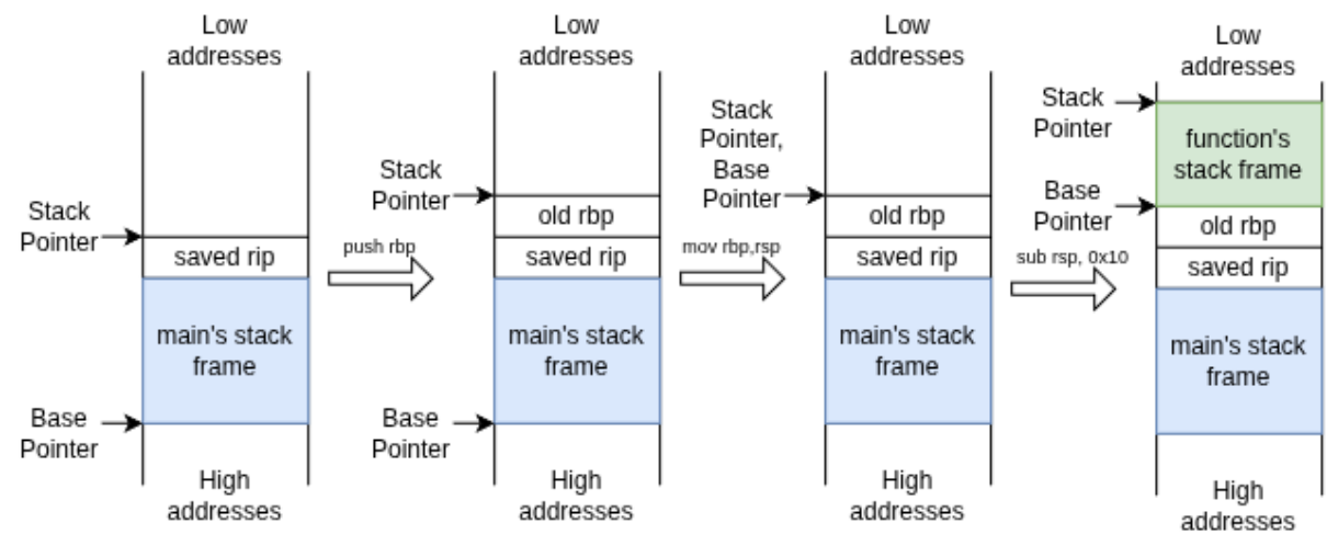
Figure 1.8: Example of what happend during a function call
