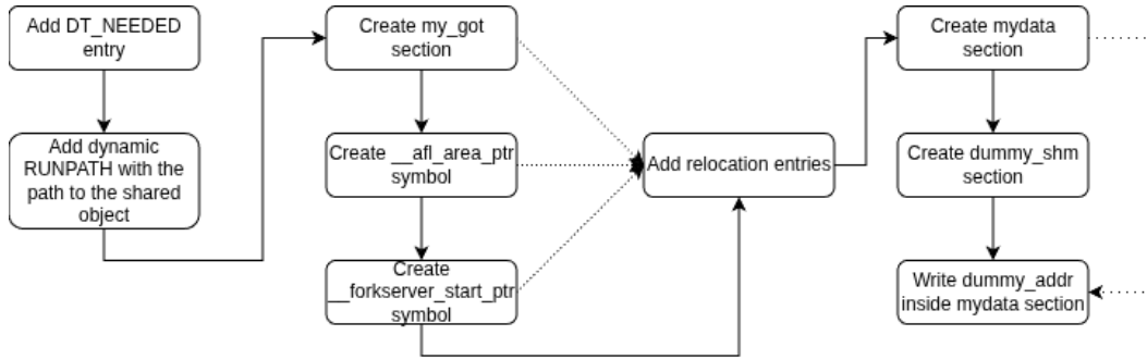
Figure 3.1: Binary modification phase in which the needed sections, relocations and dynamic dependencies are added. (The dotted arrows specify which information are needed to following steps)
