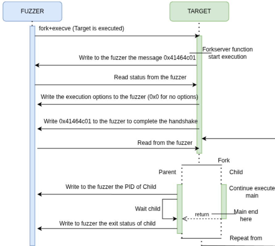
Figure 1.3: AFL++ Forkserver Protocol
