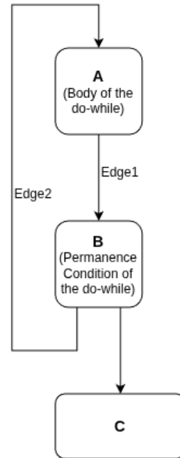
Figure 1.2: Do-while CFG
