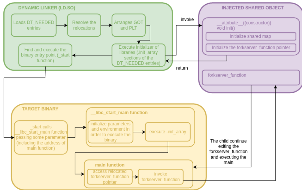
Figure 2.4: Optimized forking invocation
