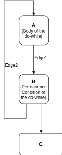
Figure 1.8: Do-while CFG
