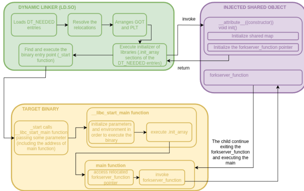
Figure 2.4: Optimized forkingserver invocation
