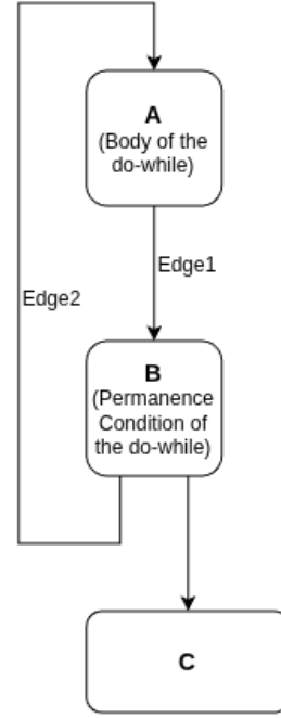
Figure 1.8: Do-while CFG
