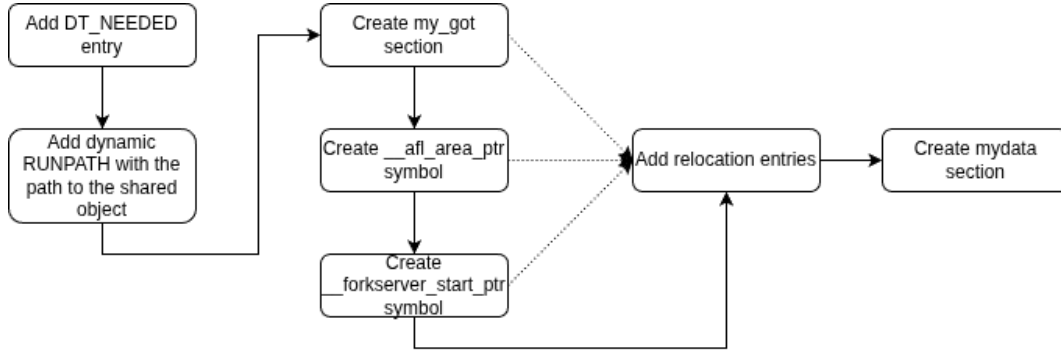
Figure 3.1: Binary modification phase in which the needed sections, relocations and dynamic dependencies are added. (The dotted arrows specify which informations are needed for the relocation phase)
