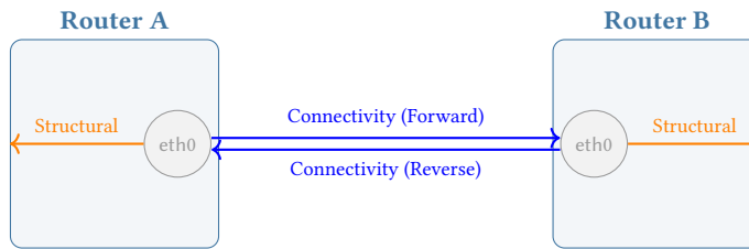
Figure 4. The Three-Hop Connectivity Pattern. To traverse from Router A to Router B, the path is: Router A Structural eth0 Connectivity eth0 Structural Router B. A bidirectional link is stored as two explicit directed Connectivity edges.
