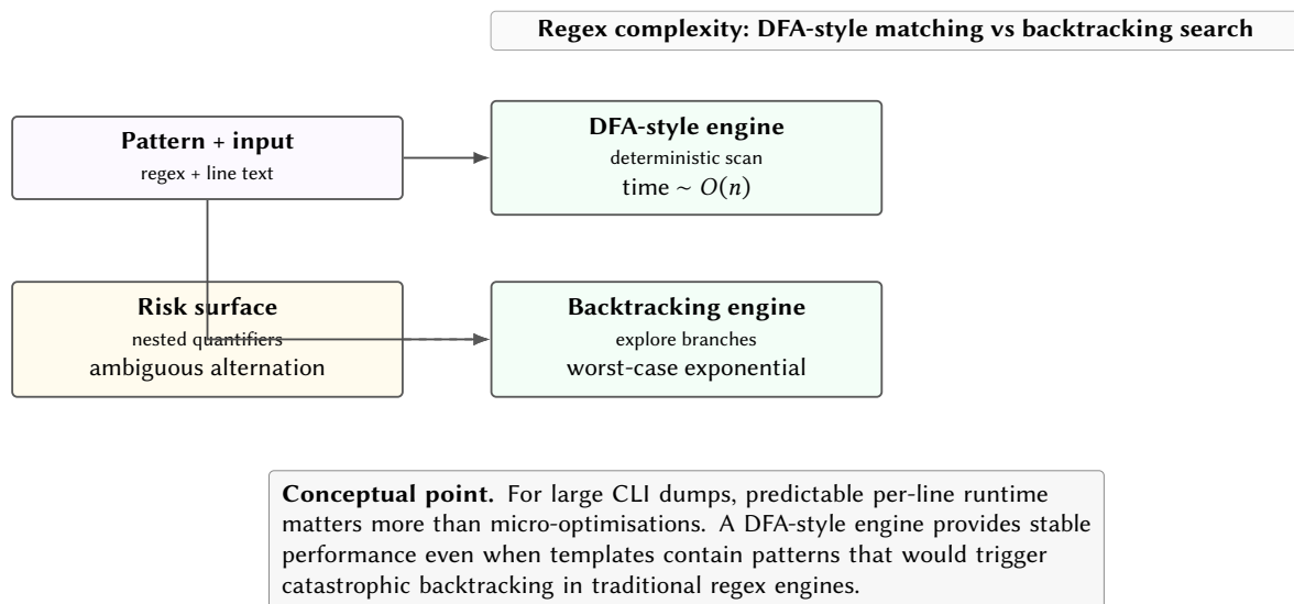
Figure 3. Why the regex engine choice matters. DFA-style matching keeps runtime predictable on long inputs, while backtracking engines can blow up on certain pattern classes.
