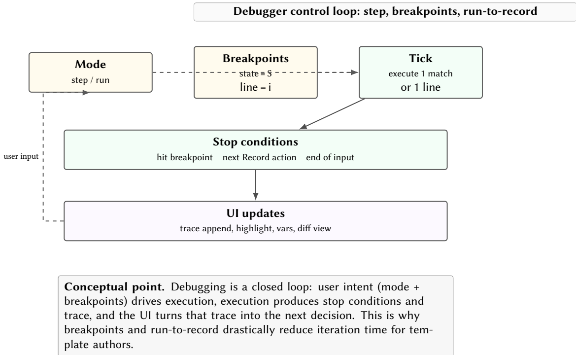
Figure 6. Debugger as a control loop over the parsing interpreter. The same trace that explains failures also drives interactive navigation (step/run/breakpoints).
