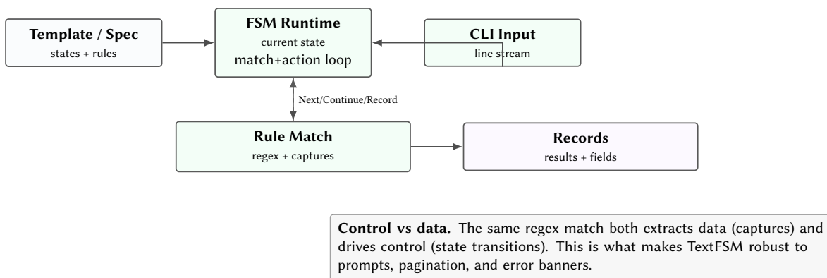
Figure 1. FSM engine model: rule matching is both evidence extraction and control-flow.
