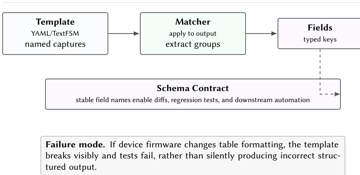
Figure 4. Templates define the parsing contract: semistructured CLI output becomes stable, typed records.
