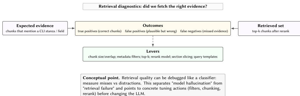
Figure 16. A practical mental model for RAG tuning. Treat retrieval as a classification problem over evidence chunks and tune for fewer false negatives (missed docs) and false positives (distractors).
