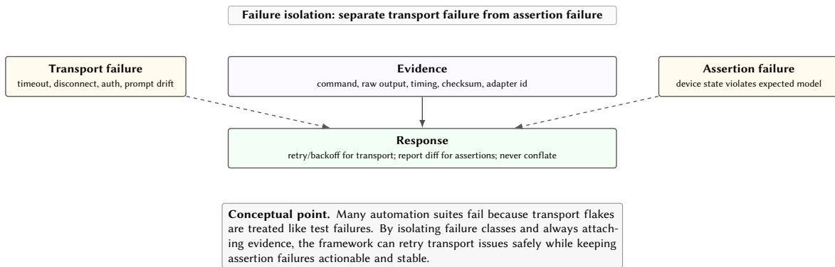
Figure 4. Failure isolation model. Transport failures trigger policy-driven retries; assertion failures produce domain-focused diffs, both grounded by the same evidence trail.
