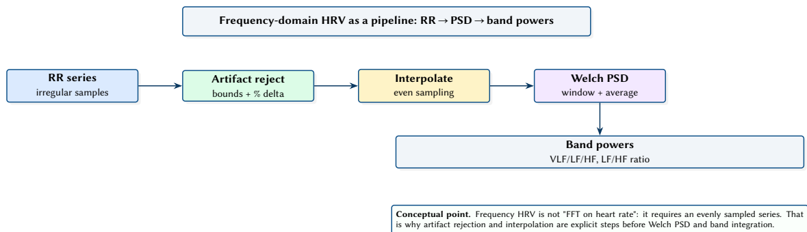
Figure 2. Frequency-domain HRV computation as a staged pipeline. Each stage exists for a reason: clean RR, resample evenly, estimate PSD robustly, then integrate band powers.
