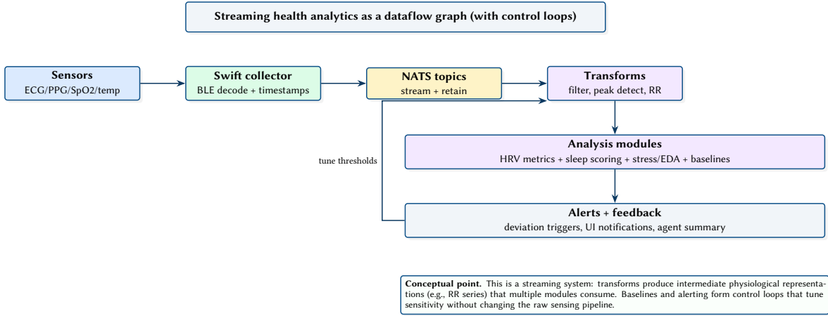
Figure 1. HealthyPi as a streaming analytics graph. Data flows through collection and transforms into multiple analysis modules, with baselines/alerts providing feedback control over sensitivity.
