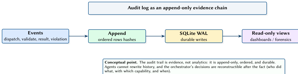
Figure 4. Append-only audit chain. Durable ordering makes the system debuggable and supports post-incident forensics without trusting agent containers.
