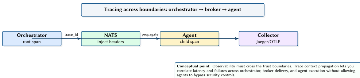
Figure 5. Distributed tracing across the orchestrator–broker–agent chain. Trace context propagates via message headers, enabling end-to-end latency attribution.
