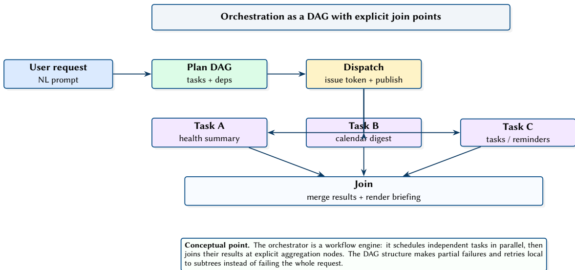
Figure 2. LLM-planned workflows as DAGs. Parallel branches run independently under capability gating, and explicit join points combine results into a final response.
