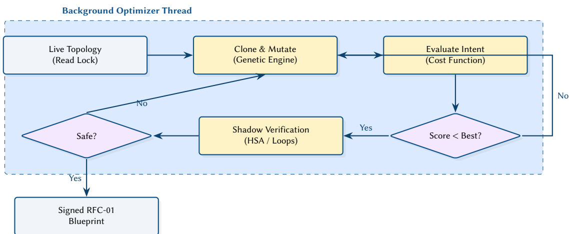
Figure 34. The Continuous Intent-Based Networking (IBN) background loop evaluating genetic mutations against declarative intents.
