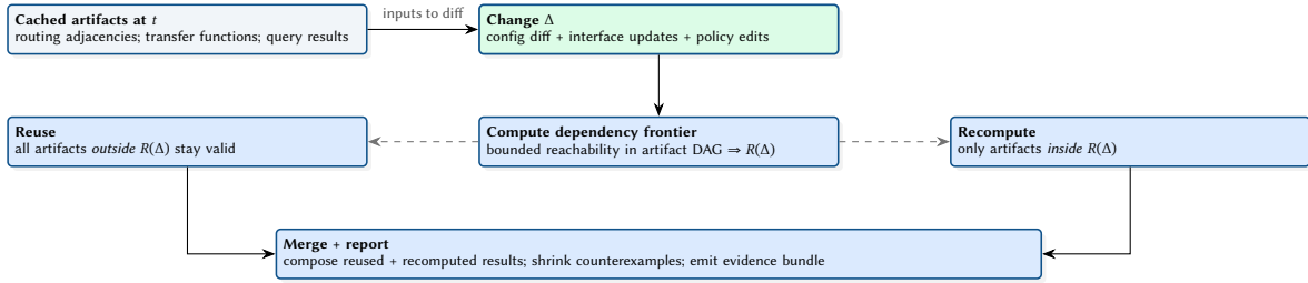
Figure 7. Algorithmic view of incremental verification. The key step is computing a dependency frontier: a bounded region R(\Delta) in the artifact dependency DAG activated by a local change. NetAssure reuses cached semantics outside the frontier and recomputes only inside it, then merges results into a single evidence bundle.
