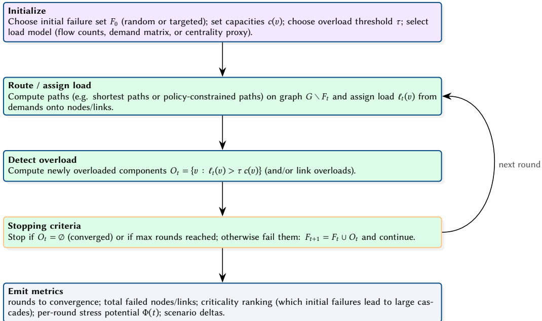
Figure 25. Cascade Monte Carlo algorithm as a deterministic inner loop wrapped by randomised initial conditions. The key design choice is the load model: it must be cheap enough to run for thousands of trials, but faithful enough to reproduce rerouting-induced overload cascades.
