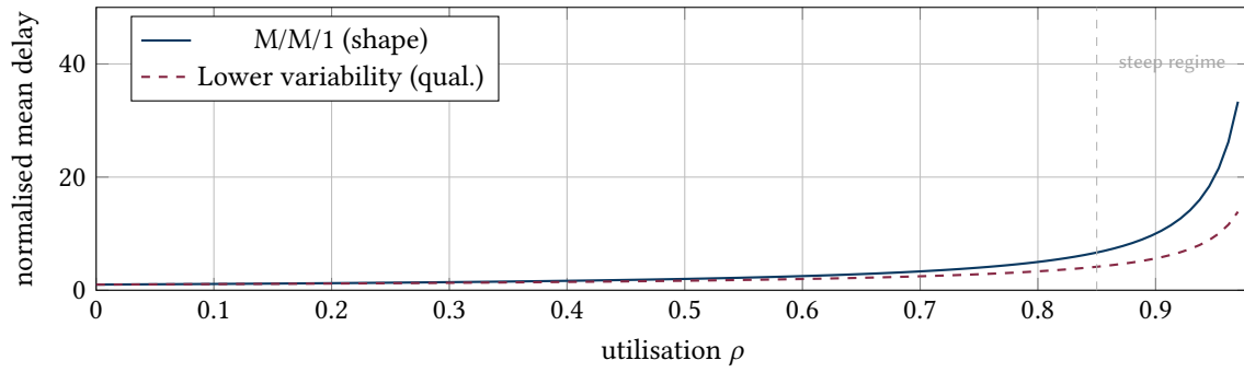
Figure 3. Non-linear delay growth near saturation. The key qualitative behaviour is the sharp increase as \rho \rightarrow 1 , which makes transient overload windows disproportionately risky.
