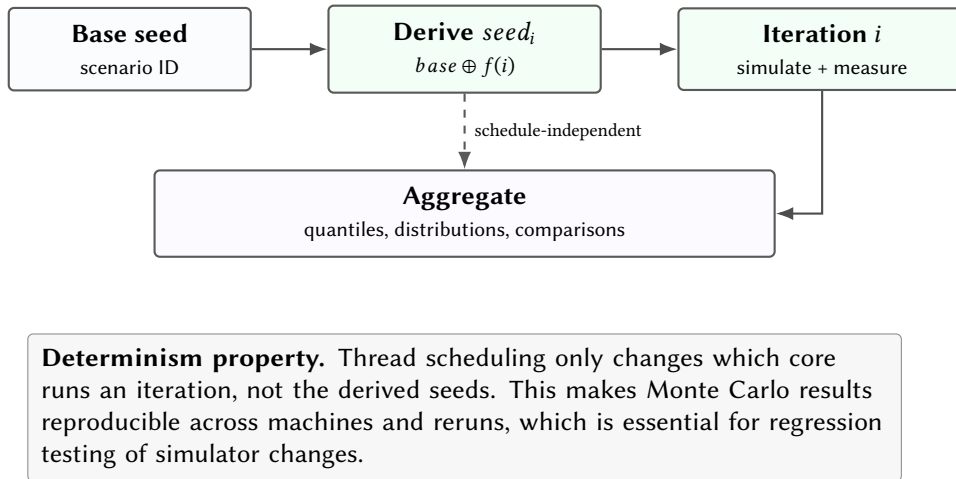
Figure 8. Deterministic Monte Carlo dataflow. The key idea is decoupling iteration identity from execution order so parallelism does not affect outcomes.
