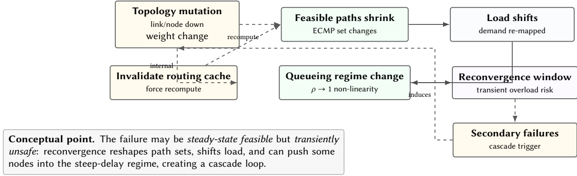
Figure 6. Routing under failure as a causal loop. Cache invalidation is an internal mechanism; reconvergence is the external risk window where non-linear queueing effects can trigger cascades.
