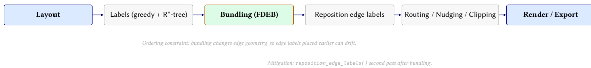
Figure 14. Refiner ordering constraint: edge bundling is geometry-changing, so it is followed by an explicit edge-label reposition pass. This keeps the pipeline composable while preserving legibility.
