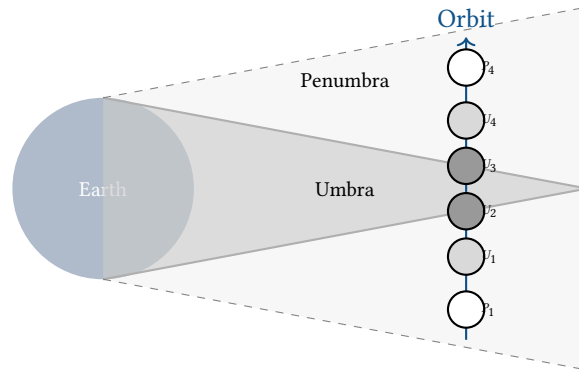
Figure 7. Lunar eclipse shadow geometry showing the Earth’s umbral and penumbral cones. The SDK predicts contact points ( P_1, U_1, U_2 , etc.) by stepping through the Moon’s geocentric ecliptic coordinates.
