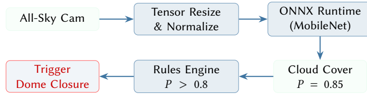
Figure 49. The Sentinel Safety Engine pipeline. Real-time imagery is processed via a cross-platform ONNX inference runtime. The resulting classification probabilities are evaluated against user-defined TOML rules to trigger emergency hardware shutdowns.
