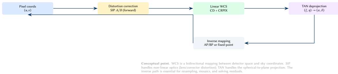
Figure 28. WCS/SIP as a bidirectional mapping. Forward maps pixels to sky coordinates; inverse maps sky to pixels for resampling and mosaic planning.
