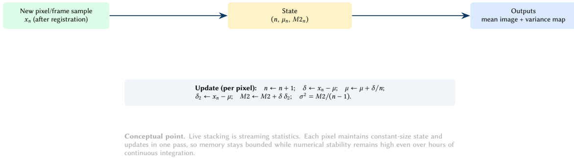
Figure 37. Welford live stacking as a streaming estimator. The system updates mean and variance online per pixel without retaining the full history.
