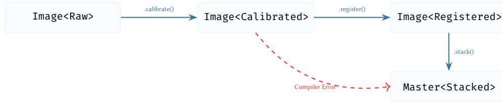
Figure 31. The Typestate pattern enforces the astrophotography pipeline at compile-time. The stack() method is only implemented for the Image<Registered> state, making it mathematically impossible to execute pipeline stages out of order.
