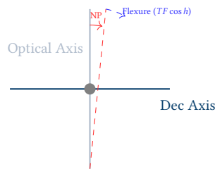
Figure 40. Mount Kinematics. The pointing model corrects for six fundamental mechanical errors: Index errors ( IH , ID ), Polar Elevation/Azimuth ( ME , MA ), Non-perpendicularity ( NP ), and Tube Flexure ( TF ).
