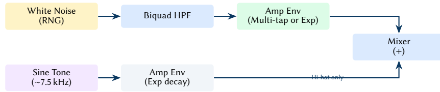
Figure 19. Percussion synthesis model. Hi-hats blend filtered noise with a metallic sine tone, while the clap relies entirely on a multi-tap noise envelope.
