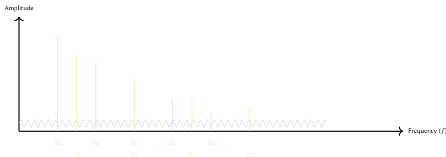
Figure 70. Harmonic spectrum of the Tanpura drone. The fundamental pitches (typically Sa and Pa) are accompanied by a dense series of upper partials that create a continuous, shimmering "bed" of sound. Overtone mimics this via multi-oscillator FM synthesis with slow phase modulations.
