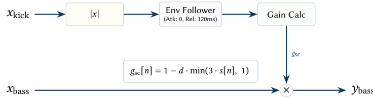
Figure 26. Sidechain compression signal flow. The absolute value of the kick signal drives an envelope follower with instantaneous attack and exponential release. This envelope calculates a dynamic gain reduction ( g_{\text{sc}} ) which is multiplied against the bass signal, ducking it to create rhythmic pumping.
