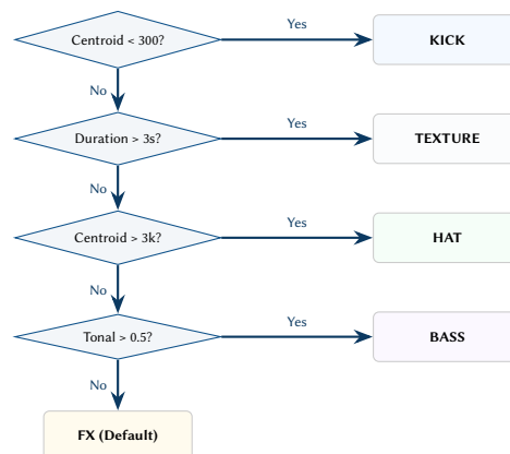
Figure 36. Rule-based sample classification decision tree. Samples are categorized using spectral and temporal heuristics. For example, low spectral centroids (< 300 Hz) combined with short attacks classify as Kicks, while high tonal scores (> 0.5) classify as Bass.
