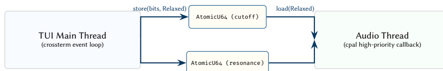
Figure 91. Lock-free concurrency model. The UI thread communicates with the real-time audio thread strictly through atomic variables, preventing priority inversion and guaranteeing that the audio callback never blocks waiting for a mutex.
