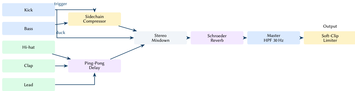
Figure 23. Master effects signal flow. The kick triggers the sidechain compressor which ducks the bass. Hi-hat, clap, and lead pass through the ping-pong delay before joining the stereo bus.
