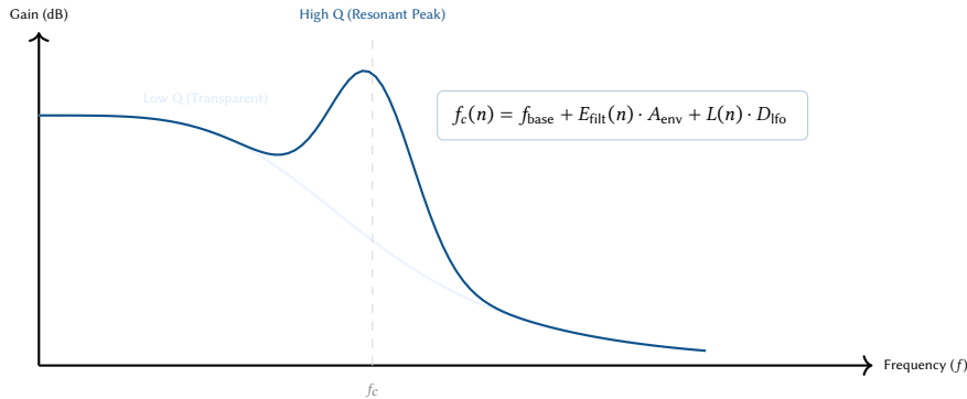
Figure 17. Filter response geometries and modulation sources. The "Acid" character is achieved by a sharp resonant peak at the cutoff frequency ( f_c ). This frequency is dynamically modulated per-sample by the filter envelope and LFO.
