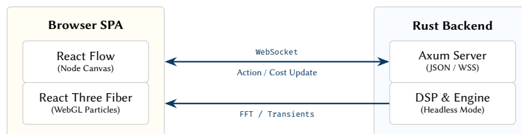
Figure 102. The Web UI Architecture. The Rust backend runs headless, exposing an Axum server. The React frontend syncs the Timeline state via WebSockets. The audio engine streams FFT and transient data directly to the Three.js particle system for zero-latency audio-reactive visuals.
