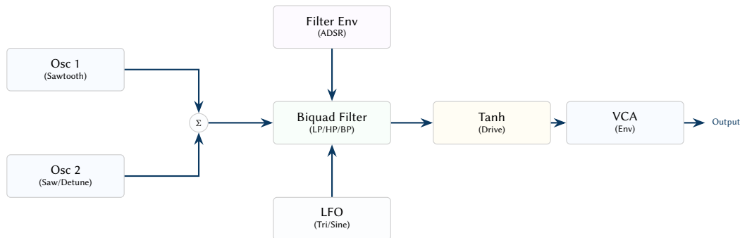
Figure 16. The bass synth signal flow. Dual sawtooth oscillators are summed and passed through a multi-mode biquad filter. Cutoff frequency is modulated by both an ADSR envelope and a free-running LFO. The signal is then saturated via a tanh function and shaped by the VCA envelope.
