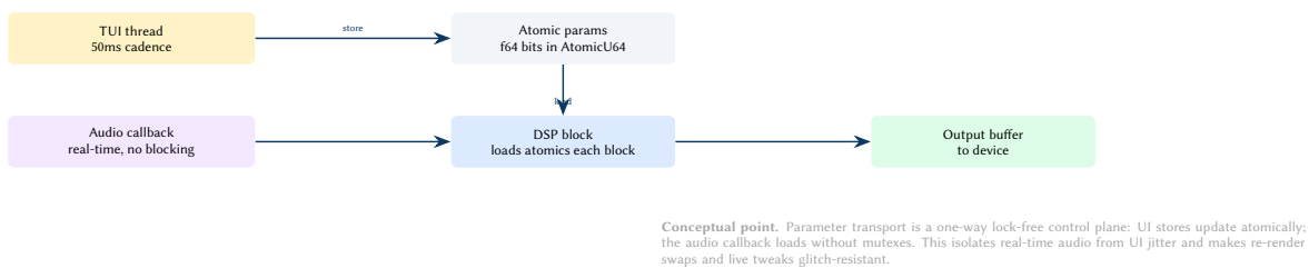
Figure 90. Lock-free control plane between UI and audio threads. Atomics carry parameters across threads without blocking the audio callback.
