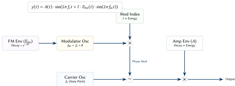
Figure 20. Two-operator FM Synthesis architecture and time-domain equation. The modulator oscillator frequency ( f_m ) is a ratio ( R ) of the carrier pitch. The modulation depth (Index I ) is dynamically scaled by the macro energy level.
