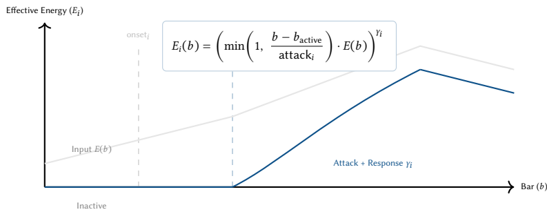
Figure 12. Sub-channel gating logic. The element remains silent ( E_i = 0 ) until both the bar onset and global energy threshold are met. Once active, the energy is scaled by a linear attack ramp and a non-linear power-law response \gamma_i .
