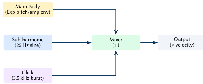
Figure 15. Kick drum synthesis model: parallel summation of main body, sub-harmonic, and click layers.
