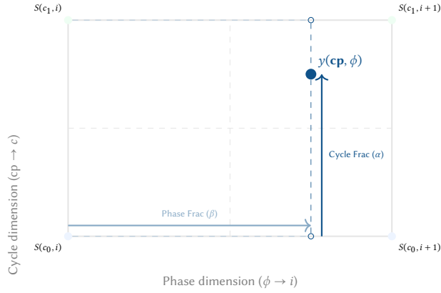
Figure 29. Bilinear cross-cycle interpolation in the Wavetable Oscillator. To prevent zipper noise when sweeping wavetables and aliasing when playing high pitches, the engine first interpolates horizontally between adjacent samples ( i and i + 1 ) within two adjacent wave cycles ( c_0 and c_1 ), and then interpolates vertically between the resulting values.
