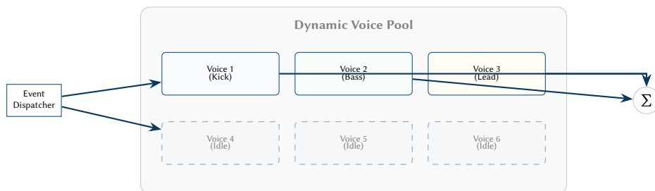
Figure 85. Dynamic voice pool management. The engine maintains a pool of pre-allocated DSP voices. When an event is dispatched, an idle voice is activated and assigned a synthesis model. Once the amplitude envelope reaches silence, the voice returns to the idle state, minimizing real-time allocations.
