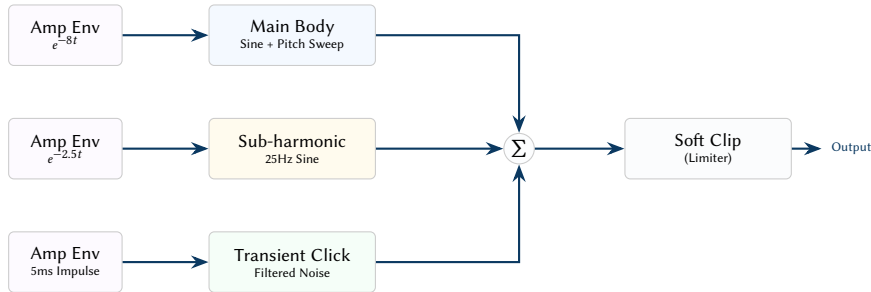
Figure 14. Three-layer kick drum synthesis architecture. The kick is synthesized by summing a pitch-swept sine body, a low-frequency sub-harmonic, and a short-duration noise click for transient definition. Each layer has an independent amplitude envelope scaled by the humanization engine.
