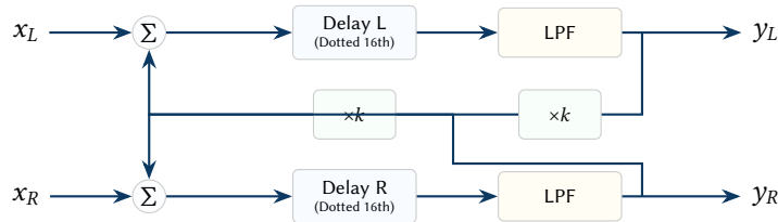
Figure 27. Ping-Pong Delay topology. Left and right channel inputs ( x_L, x_R ) are fed into independent delay lines. The output of each delay line is low-pass filtered (for analog-style damping), multiplied by the feedback coefficient k , and routed into the input sum of the opposite channel's delay line, creating a stereo bouncing effect.
