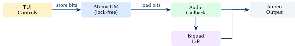
Figure 87. Lock-free live parameter path: the TUI stores f64 bit patterns into atomics; the audio callback loads them each block and updates the biquad filter only when thresholds are exceeded.
