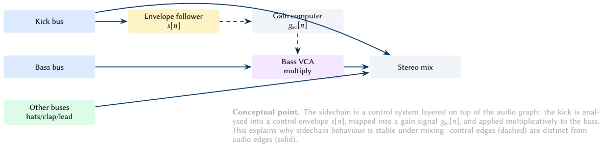
Figure 24. Sidechain compression as a control graph. Dashed arrows carry control signals; solid arrows carry audio. This framing clarifies how the kick shapes bass dynamics without being mixed into the control path.
