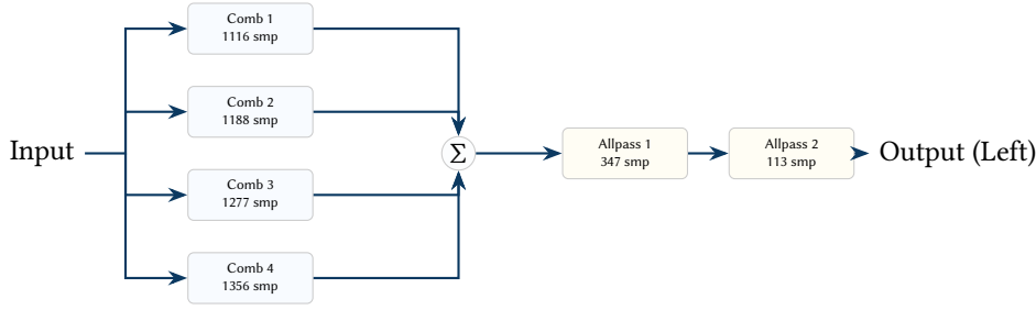
Figure 28. Schroeder Reverb topology (Left Channel). The input signal is fed in parallel to four comb filters with mutually prime delay lengths. Their outputs are summed and passed serially through two allpass filters to increase echo density without coloring the sound.
