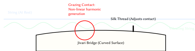
Figure 69. The Jivari bridge mechanism. The bridge has a slightly curved top surface. As the string vibrates, it grazes the bridge at varying points along its length. This periodic "buzzing" creates a rich, non-linear series of overtones. Overtone approximates this shimmer using FM synthesis with a high modulation index.
