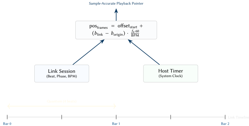
Figure 81. Ableton Link phase-locked synchronisation. The engine maps the shared Link timeline (beats) to local audio buffers using the system’s high-precision timer. Playback is quantized to 4-beat boundaries, ensuring that Overtone’s kick drum aligns perfectly with external peers.
