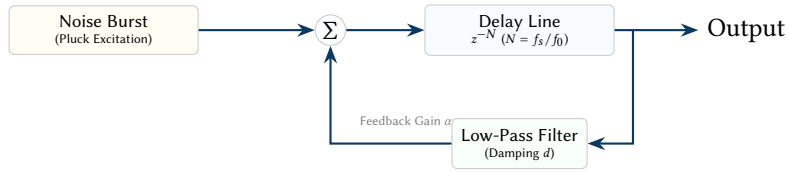
Figure 22. Karplus-Strong physical modeling architecture. A short burst of noise (the "pluck") is fed into a delay line representing the string length. The output is fed back through a low-pass filter, causing higher frequencies to decay faster than fundamental frequencies, realistically simulating a plucked acoustic string.
