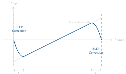
Figure 31. PolyBLEP discontinuity correction. The "naive" sawtooth waveform has an infinite slope at the wrap-around point, which creates aliases across the entire frequency spectrum. The PolyBLEP algorithm subtracts a band-limited residual (the BLEP) within one sample period ( \Delta t ) of the discontinuity, effectively smoothing the edge and suppressing digital artifacts.
