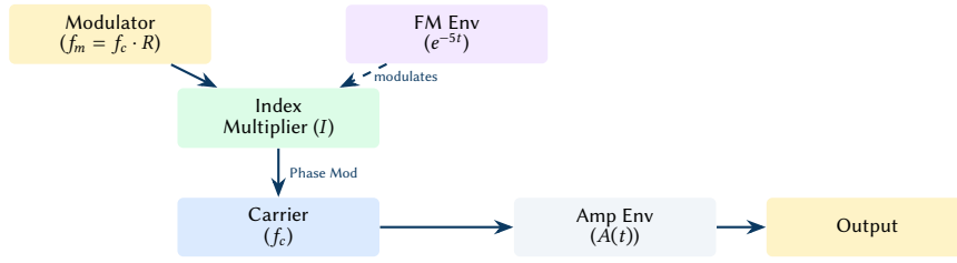
Figure 21. Lead synthesiser signal flow using 2-operator FM.
