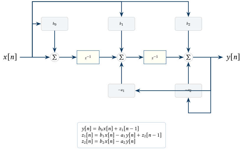
Figure 25. Biquad filter Direct Form II Transposed topology. This structure is preferred for its numerical stability and low memory footprint, requiring only two delay registers ( z_1, z_2 ) per filter instance.
