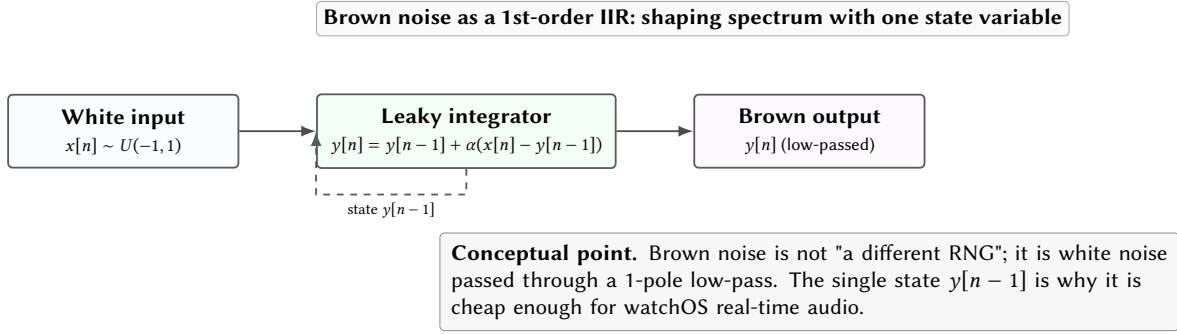
Figure 2. Brown noise generation as a minimal-state filter. One multiply-add plus one state variable shapes the spectrum toward low frequencies.
