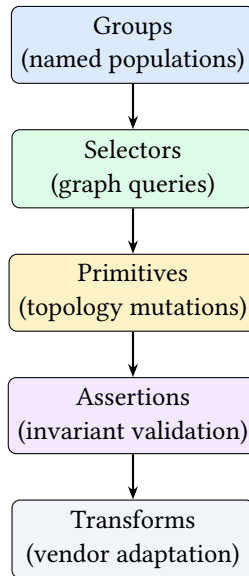
Figure 1. Lowering chain from plan-layer constructs to vendor-specific output.
