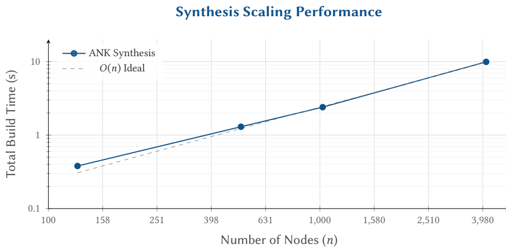
Figure 8. Synthesis Performance Metrics: ANK maintains linear complexity.
