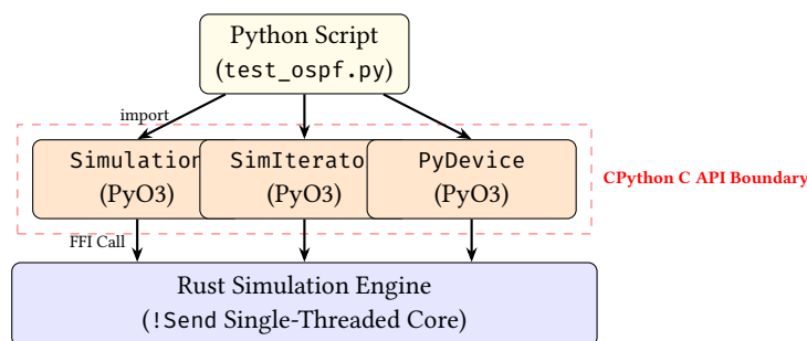
Figure 9. Python Bindings Architecture. The PyO3 wrappers expose the single-threaded Rust Engine directly to the Python interpreter, allowing zero-copy, in-process access to the simulation state.
