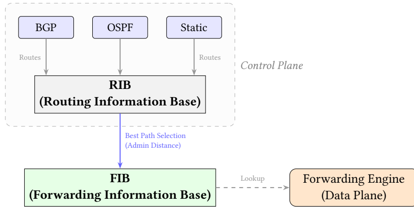
Figure 3. RIB/FIB Separation. Multiple routing protocols populate the global RIB. The router executes best-path selection based on Administrative Distance to program the active FIB used by the forwarding engine.
