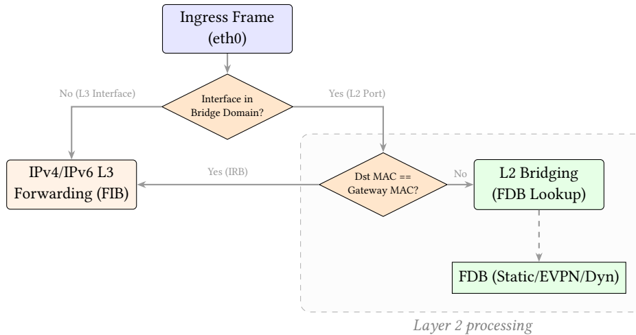
Figure 7. Unified L2/L3 Router Abstraction. Incoming frames branch based on interface bridge domain membership. IRB (Integrated Routing and Bridging) allows L2 frames addressed to the gateway MAC to seamlessly bridge into the L3 forwarding path.
