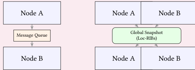
Figure 8. EVPN Snapshot Abstraction. Instead of modeling asynchronous TCP queues and individualized BGP update messages (left), netsim captures a global snapshot of all EVPN Loc-RIBs at phase P2.5 and atomically applies changes to all peers (right), guaranteeing deterministic state replication.
