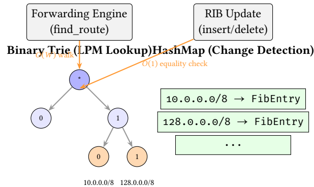
Figure 4. Dual-Index FIB Architecture. The Forwarding Engine uses the Binary Trie for fast Longest-Prefix-Match lookups, while RIB updates use the HashMap for O(1) exact-match change detection to avoid spurious convergence resets.
