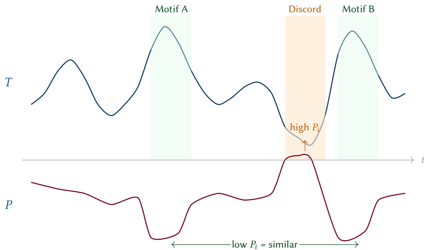
Figure 2. Conceptual overview. A time series T (top) contains a repeated motif (green) and an anomaly (orange). The Matrix Profile P (bottom, purple) assigns low distances to motif positions and high distances to the discord. Reading the profile's minima yields motifs; its maxima yield discords.
