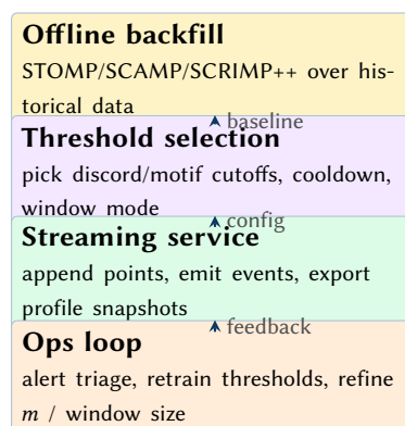
Figure 16. Operational use case loop. A common pattern is to backfill exact profiles offline, derive thresholds, then run a long-lived streaming service with periodic recalibration.
