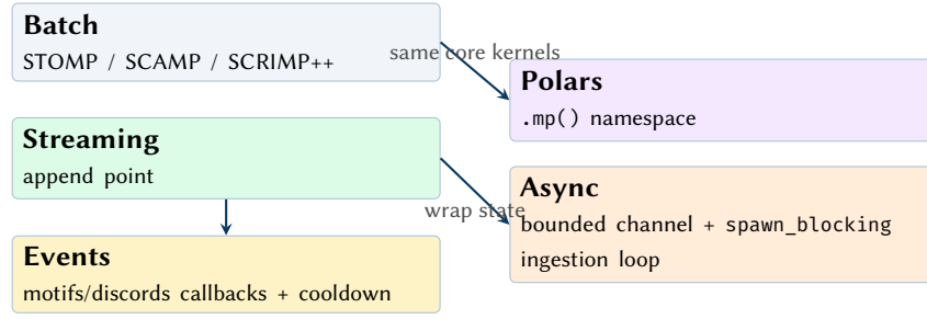
Figure 4. API at a glance. matrix-profile-rs exposes batch, streaming, and ecosystem integration entrypoints that share the same core kernels and profile representations.
