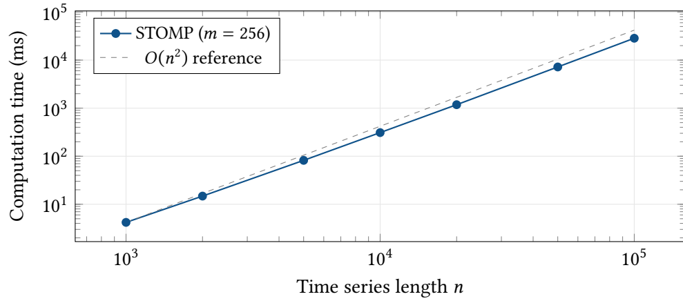
Figure 23. STOMP batch scaling. Measured times track ideal O(n^2) scaling closely across two orders of magnitude.
