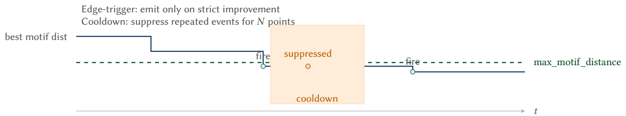
Figure 13. Notification semantics (motifs shown). Events are edge-triggered: a motif event fires only when the global best-so-far distance strictly improves past the configured threshold. A cooldown window suppresses repeated events during rapid convergence.
