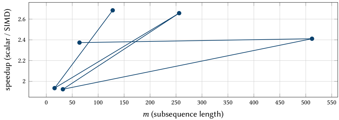
Figure 20. SIMD speedup for centered sumproducts initialisation (Criterion). Generated by make -C docs/report bench-report .
