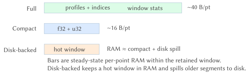
Figure 24. Memory overhead by mode (conceptual). Compact mode reduces per-point storage by narrowing statistics and profile representations; disk-backed mode caps RAM by spilling segments to persistent storage.
