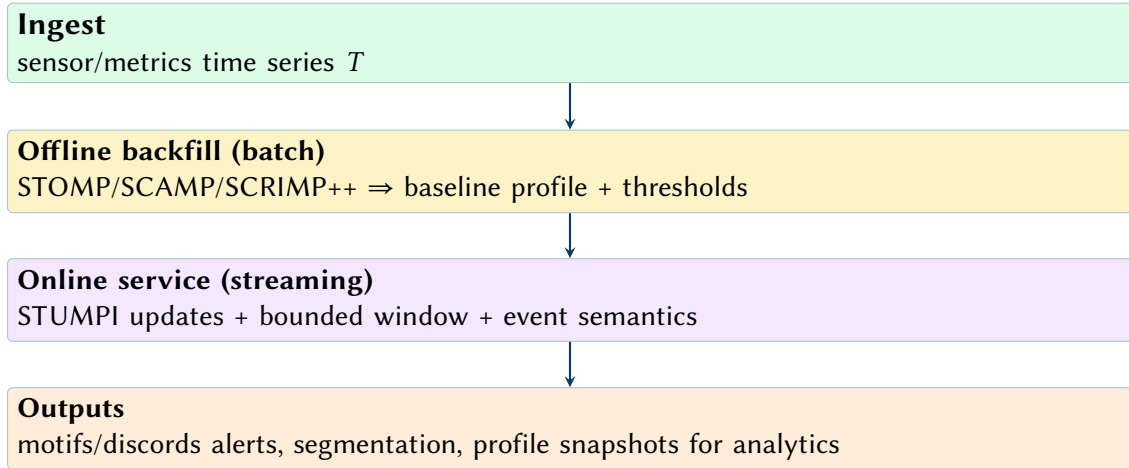
Figure 1. System overview. Batch backfill establishes baselines and thresholds; streaming maintains a sliding profile and emits events. Snapshot outputs integrate with analytics and DataFrame workflows.
