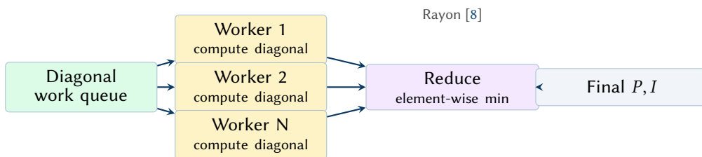
Figure 7. Parallelisation over diagonals. Each diagonal is processed independently on a Rayon worker thread; partial results are merged with an element-wise minimum reduction.
