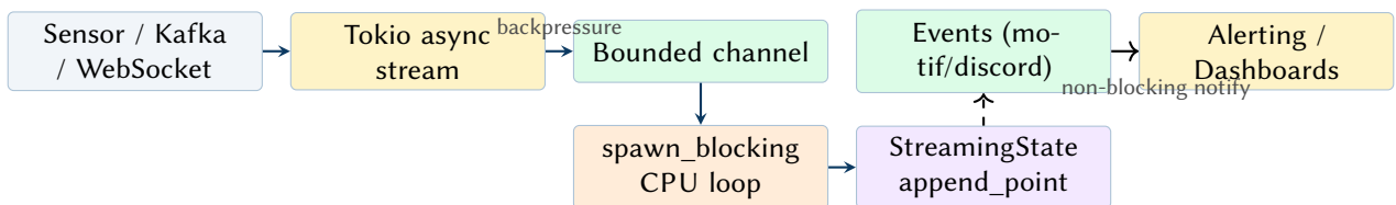
Figure 15. Async deployment pattern. An async source feeds a bounded channel; CPU-bound updates run on spawn_blocking , while event notifications are delivered without stalling ingestion.
