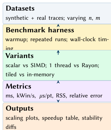
Figure 22. Evaluation methodology flow. We run controlled benchmark variants and report both throughput and correctness metrics to avoid performance-only optimisation bias.
