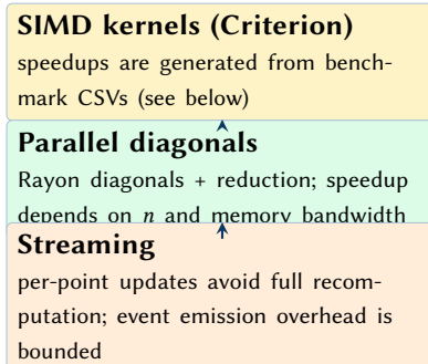
Figure 19. Observed performance effects (representative). SIMD acceleration yields large constant-factor wins in the hot inner kernels; parallel diagonal processing provides further throughput gains when memory bandwidth permits.
