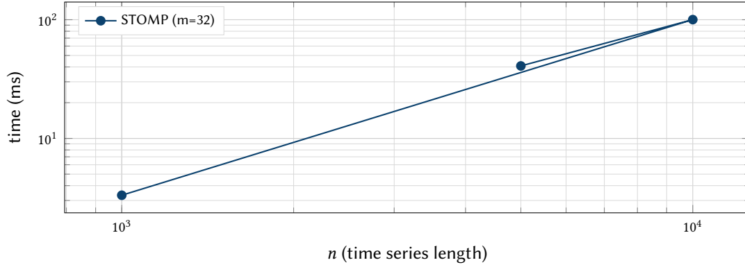
Figure 17. End-to-end STOMP scaling (Criterion, representative). Log-log axes emphasise the rapid growth in compute cost with n for exact batch joins. Values match Table 3.
