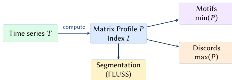
Figure 3. Matrix Profile downstream tasks. The profile vector P supports motif and discord discovery via extrema, while the index vector I supports regime change detection via FLUSS [6].
