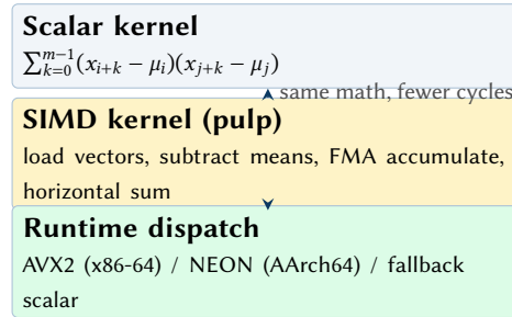
Figure 6. SIMD acceleration strategy. pulp [7] selects an optimal vectorised implementation at runtime while preserving a scalar fallback path.
