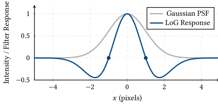
Figure 16. 1D profile of a Gaussian star (grey) and the normalized Laplacian of Gaussian (LoG) filter response (blue). The zero-crossings of the LoG function formally define the inflection edges of the star’s spatial profile, allowing for robust multi-scale star detection invariant to background gradients.
