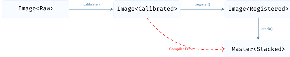
Figure 27. The Typestate pattern enforces the astrophotography pipeline at compile-time. The stack() method is only implemented for the Image<Registered> state, making it mathematically impossible to execute pipeline stages out of order.
