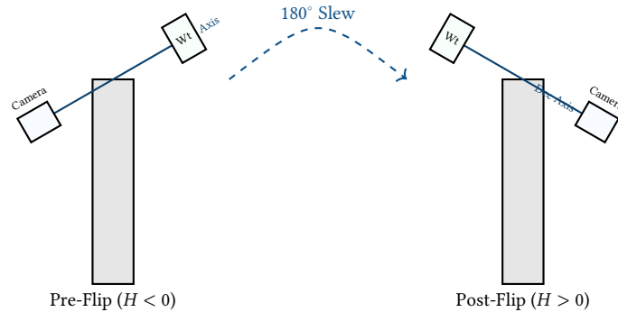
Figure 36. The Meridian Flip. To prevent collision with the pier, the orchestrator halts tracking, rotates the Right Ascension axis by 12 hours ( 180^\circ ), and reverses the Declination axis, effectively placing the camera "above" the mount.
