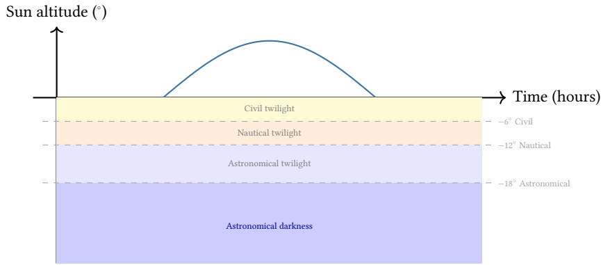
Figure 9. Twilight boundary model. The twilight_times function locates the six solar altitude crossings that delimit civil, nautical, and astronomical twilight, bounding the usable deep-sky imaging window.
