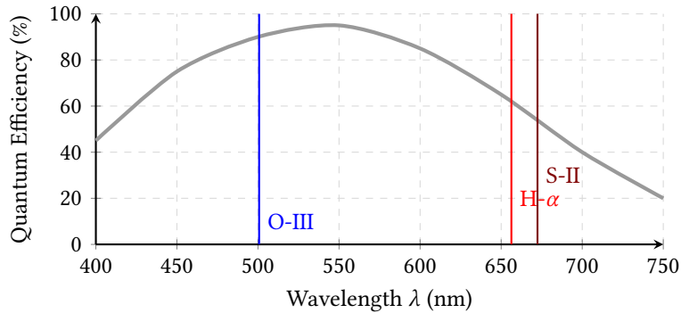
Figure 13. Quantum Efficiency curve of a typical Back-Illuminated (BSI) CMOS sensor. The noise model calculates the expected signal-to-noise ratio by integrating the target's emission spectrum against the sensor's specific QE at key narrowband wavelengths (500.7 nm, 656.3 nm, 672.4 nm).
