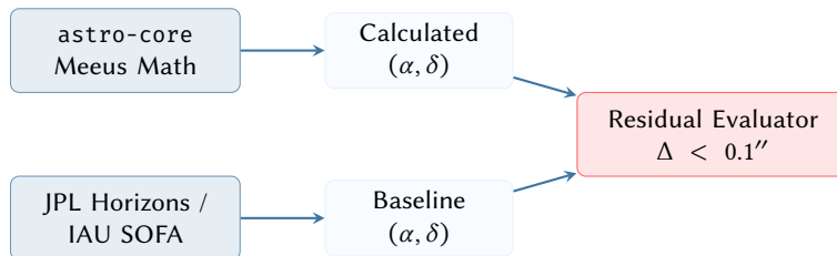
Figure 29. Golden Master CI/CD testing pipeline. The SDK's coordinate output is dynamically asserted against the gold-standard JPL Horizons ephemeris data [23] to guarantee that the implementation is free from systemic truncations or coordinate frame misinterpretations.
