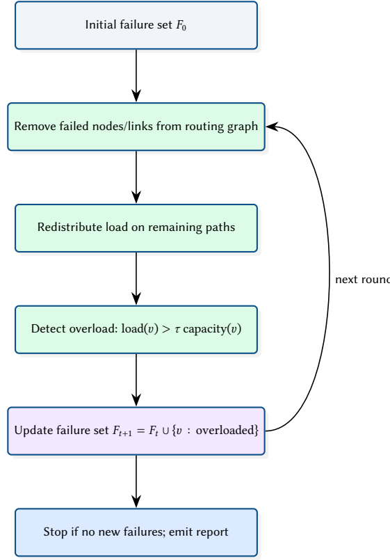
Figure 12. Round-based cascade progression used in the Monte Carlo simulator.
