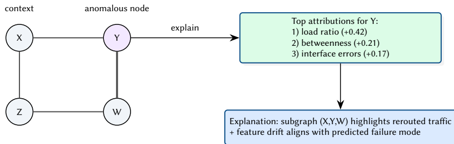
Figure 21. Conceptual explanation output: anomalous node with a small explanatory subgraph and feature attributions.
