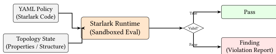
Figure 17. Starlark Policy Evaluation. The sandboxed runtime safely evaluates Python-like policy code against the topology state to generate deterministic compliance findings.
