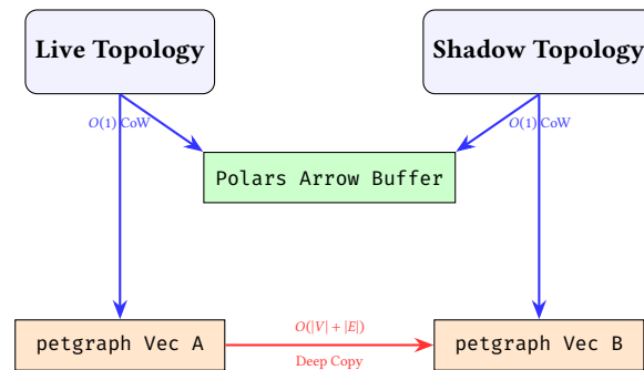
Figure 19. The Hybrid Snapshot Reality. While property DataFrames share memory efficiently via CoW pointers, the underlying petgraph adjacency lists must be physically deep-copied into new memory allocations.
