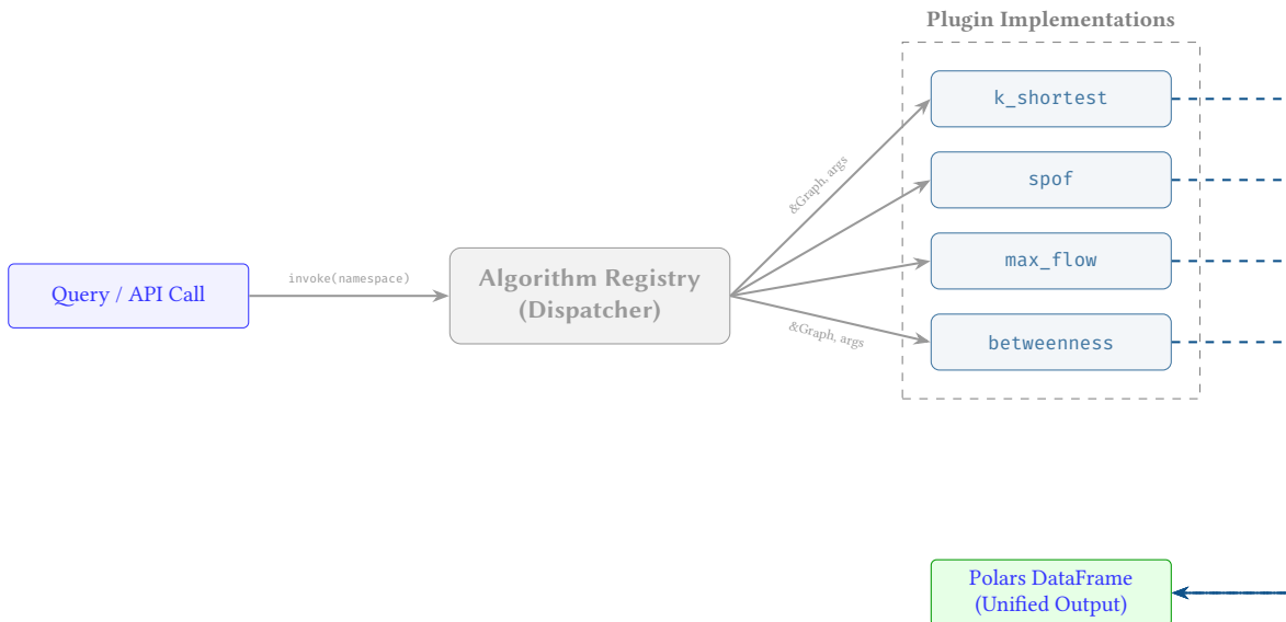
Figure 59. Graph Algorithm Plugin Architecture. The dispatcher routes calls by namespace to specific plugin kernels, which operate on a shared graph reference and uniformly return their mathematical results as structured Polars DataFrames.
